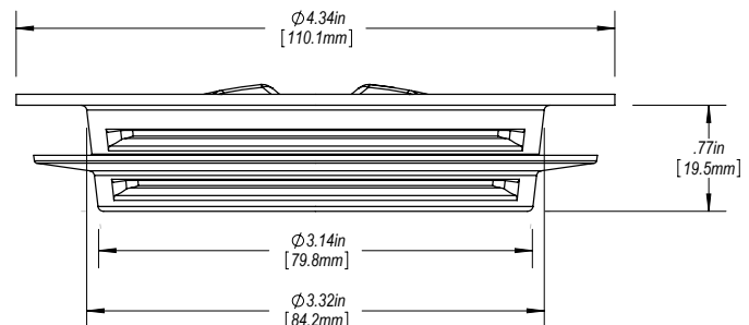
Housing & Gasket
