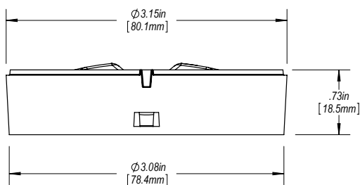
Housing (No Gasket)
