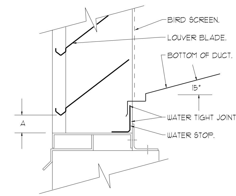
LOUVER CONNECTION DETAIL NTS
