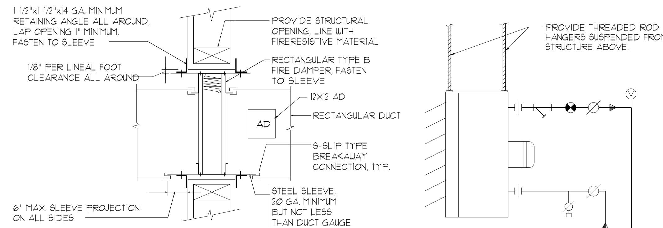
RECTANGULAR FIRE DAMPER INSTALLATION DETAIL NTS
