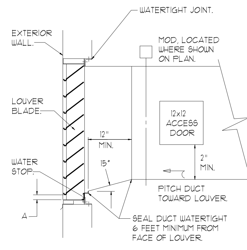
LOUVER DETAIL WITH HORIZONTAL DUCT NTS
