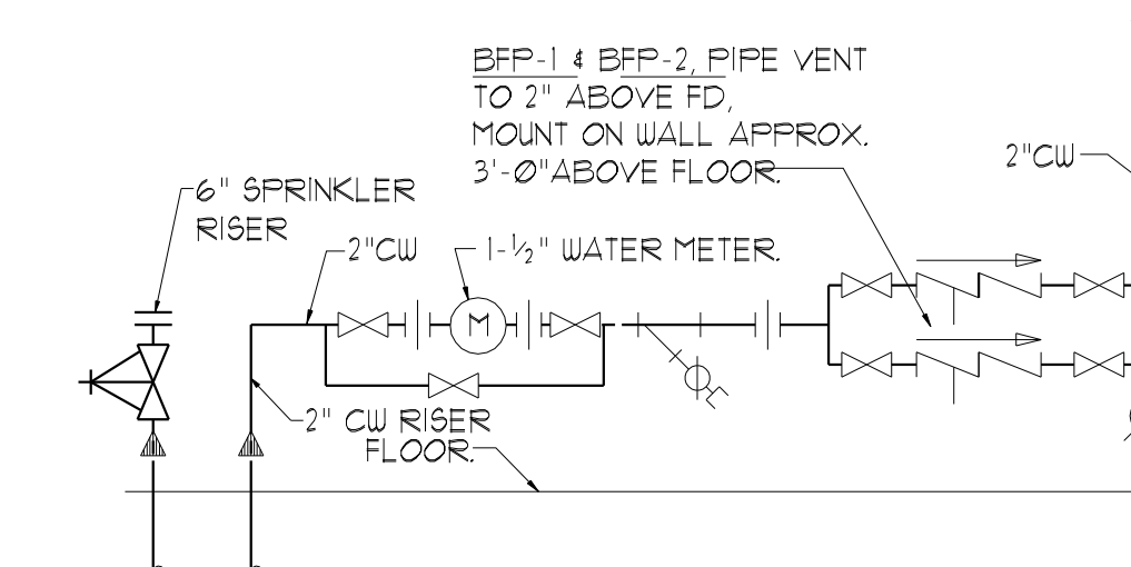
WATER ENTRANCE DETAIL NTS
