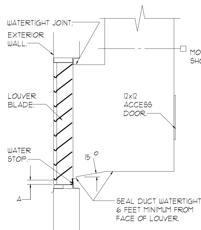
LOUVER DETAIL WITH DUCT FROM ABOVE NTS
