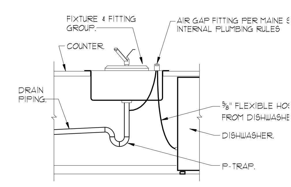
DISHWASHER DRAIN DETAIL NTS
