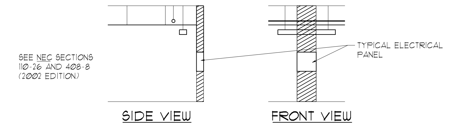
CLEARANCES AT ELECTRICAL PANELS NTS
