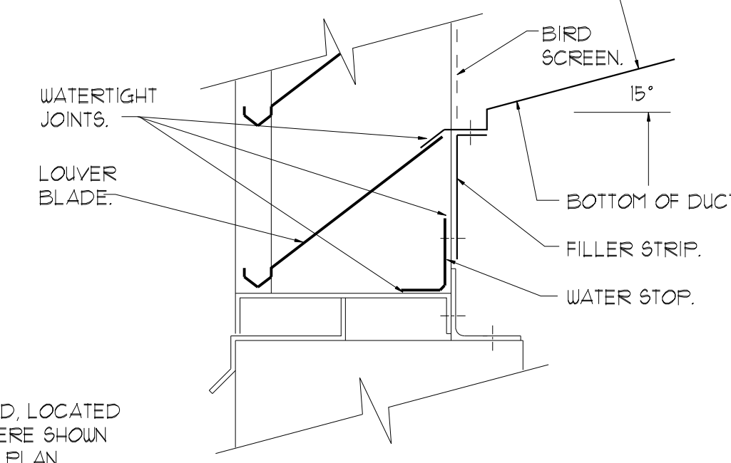
MODIFIED LOUVER DETAIL NTS
