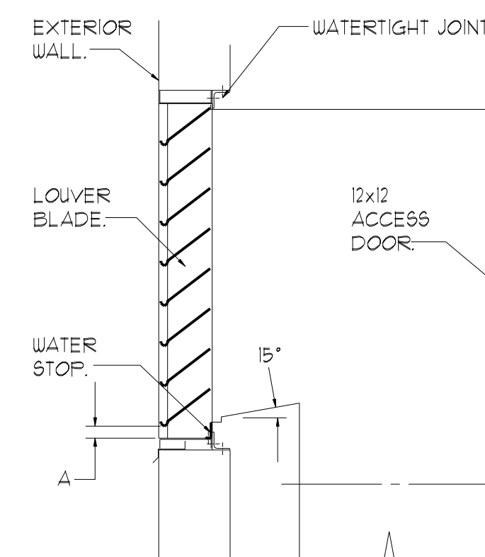
LOUVER DETAIL WITH DUCT FROM BELOW NTS
