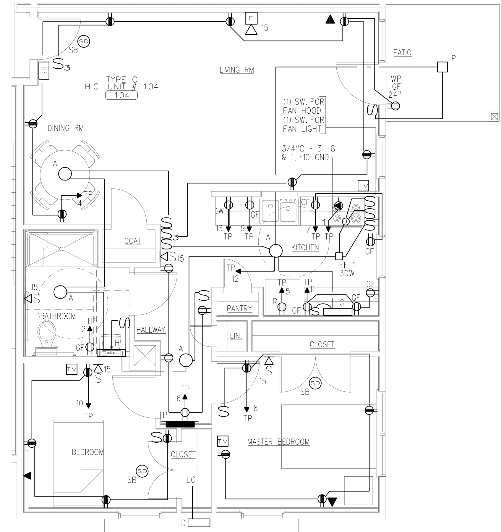
ELECTRICAL PLAN - TYPE C H.C. UNIT SCALE: 1/4" = 1'-0"
