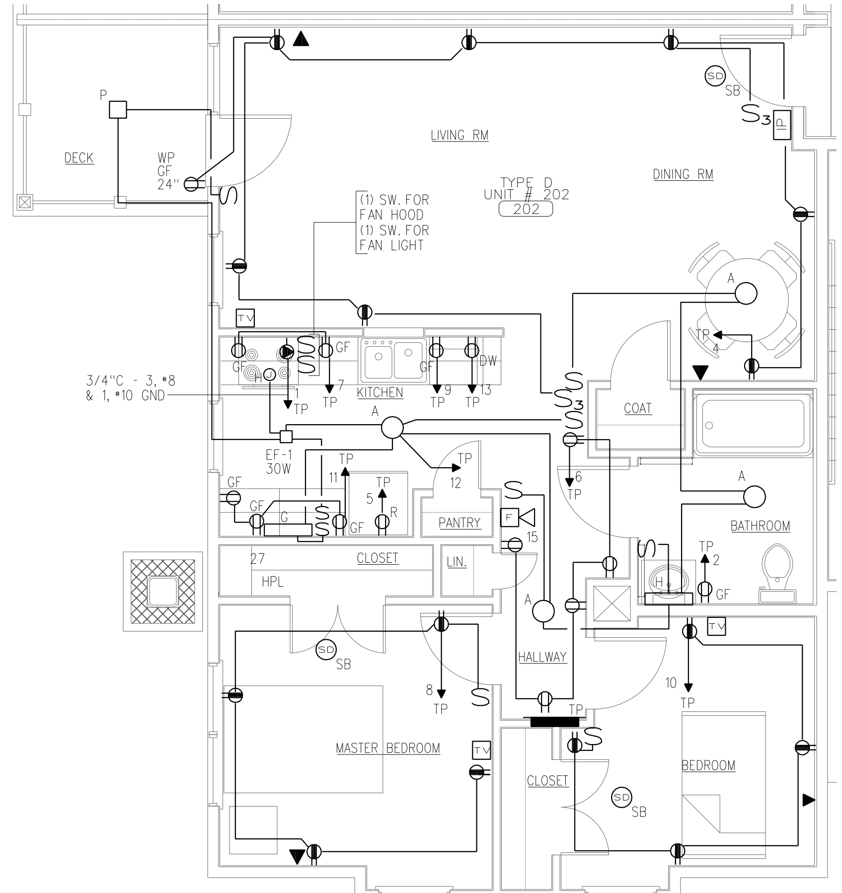
ELECTRICAL PLAN - TYPE D UNIT SCALE: 1/4" = 1'-0"
