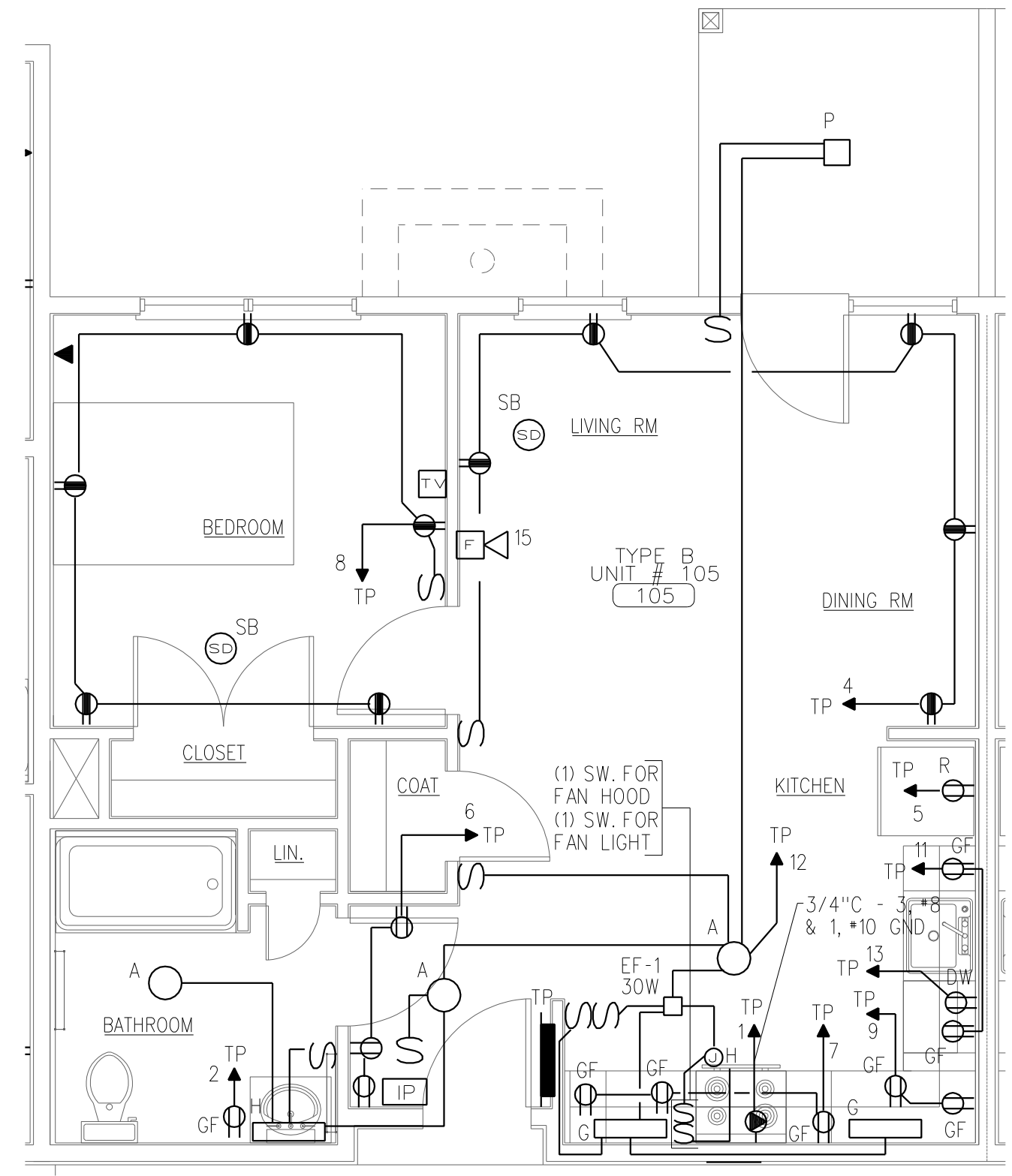
ELECTRICAL PLAN - TYPE B UNIT SCALE: 1/4" = 1'-0"
