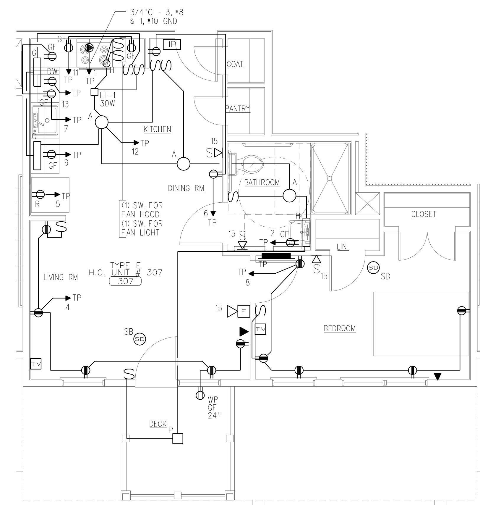
ELECTRICAL PLAN - TYPE E H.C. UNIT SCALE: 1/4" = 1'-0"
