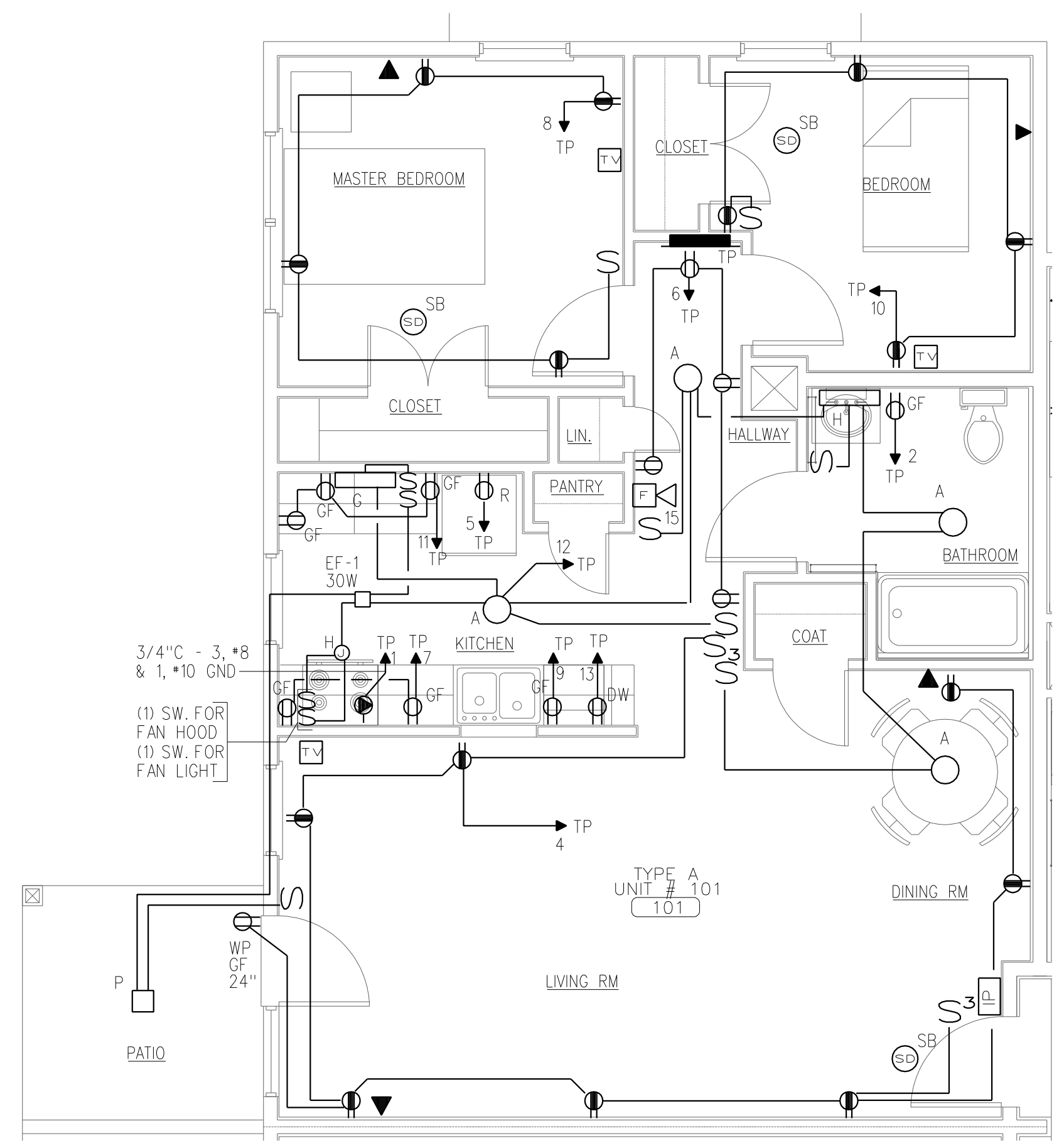
ELECTRICAL PLAN - TYPE A UNIT SCALE: 1/4" = 1'-0"
