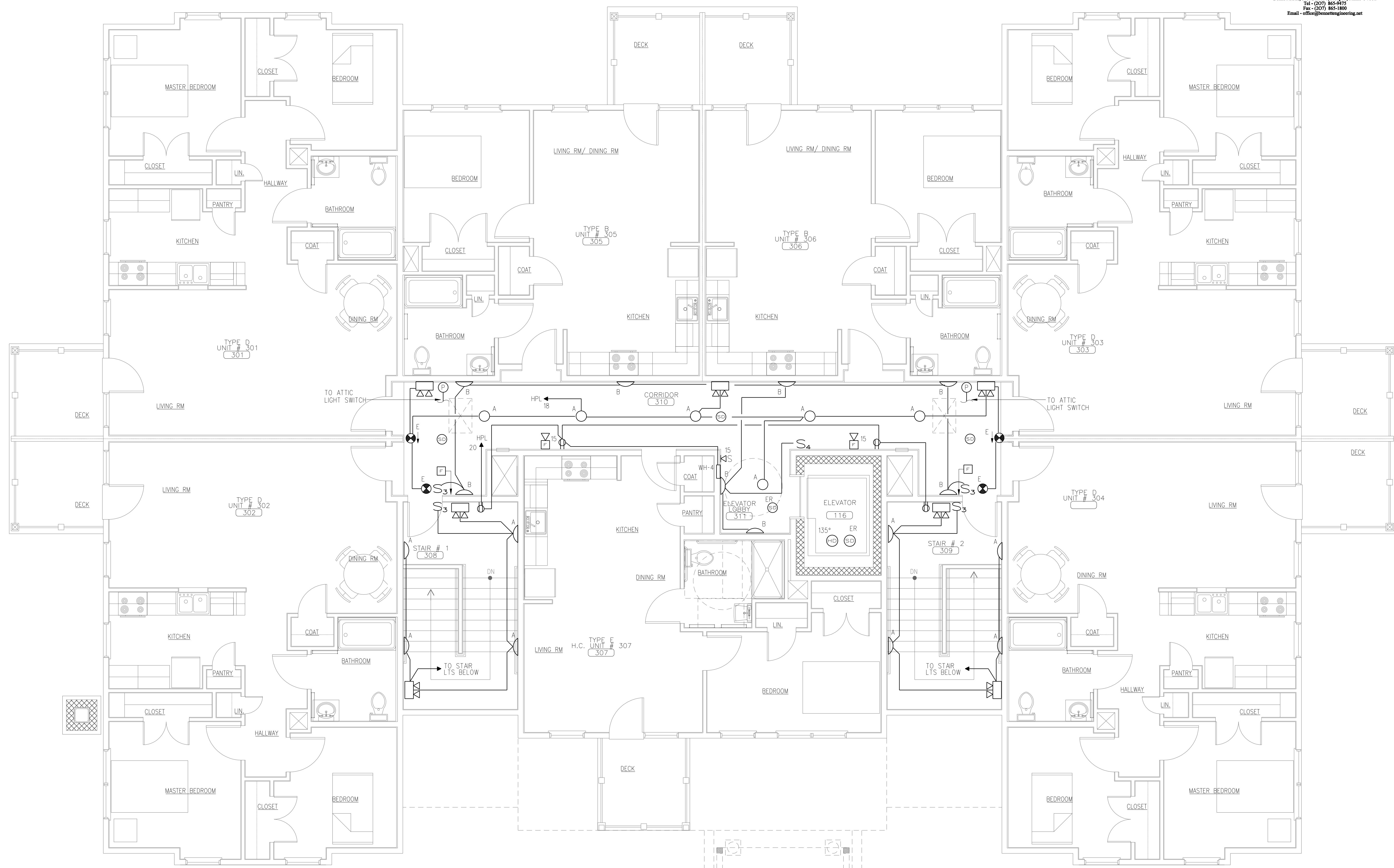
THIRD FLOOR ELECTRICAL PLAN SCALE: 1/4" = 1'-0"
