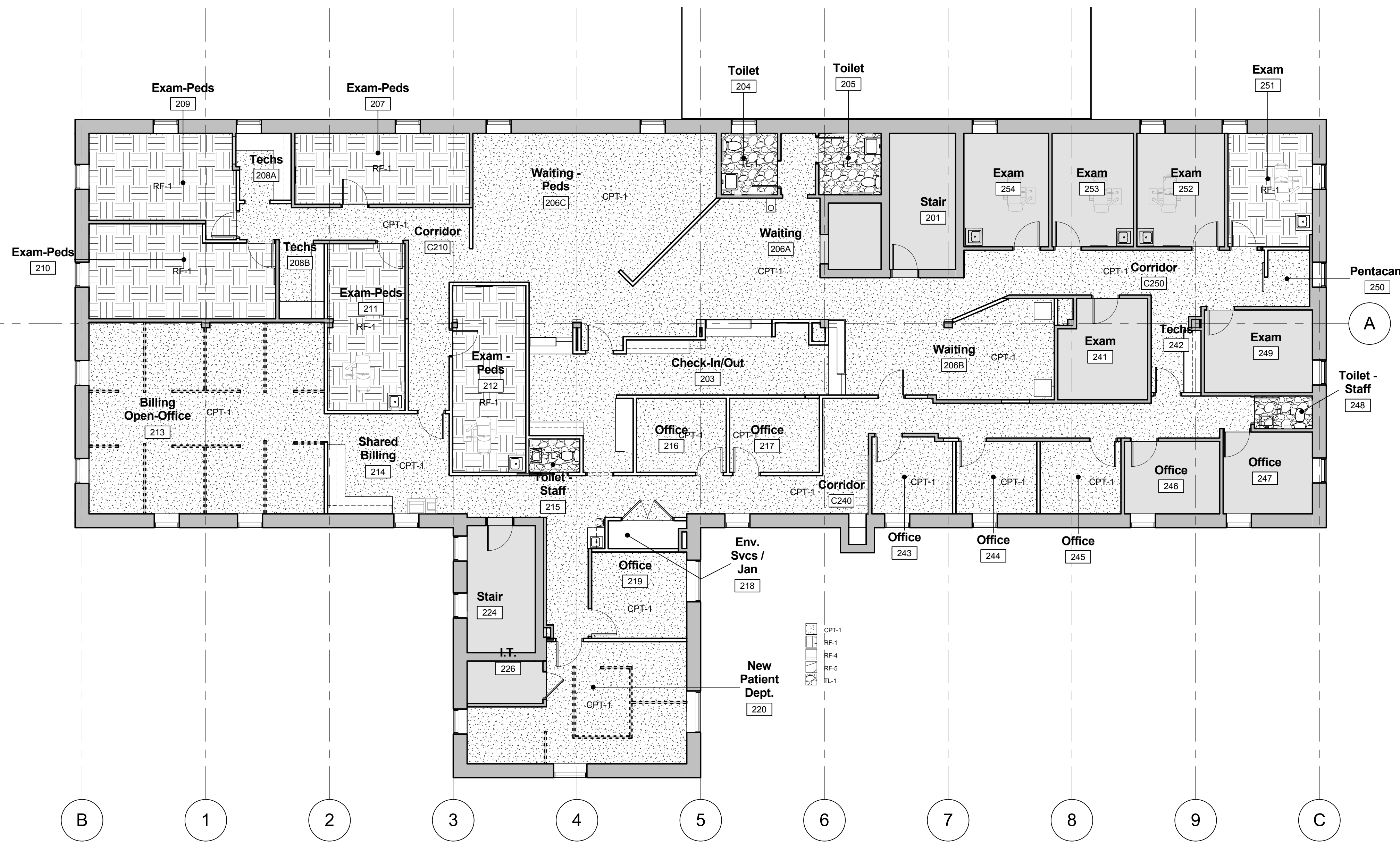
1 Level 2 - Finishes Plan 1/8" = 1'-0"
