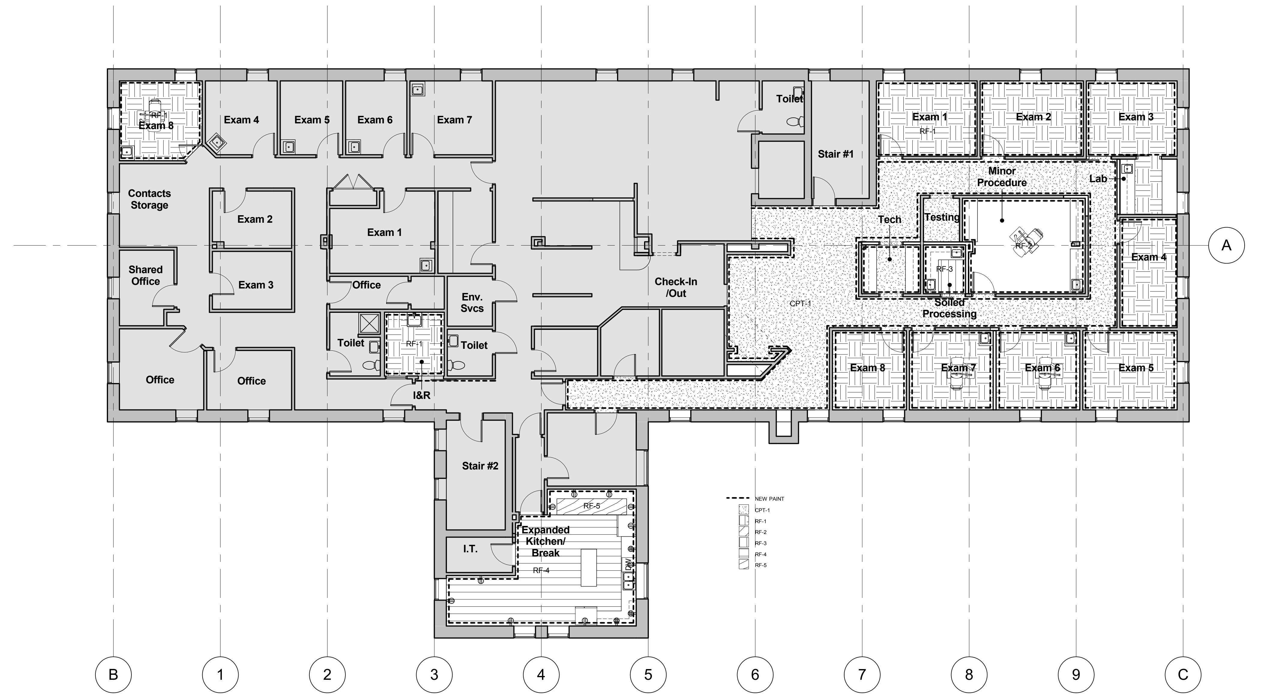
1 Level 4 - Finishes Plan 1/8" = 1'-0"
