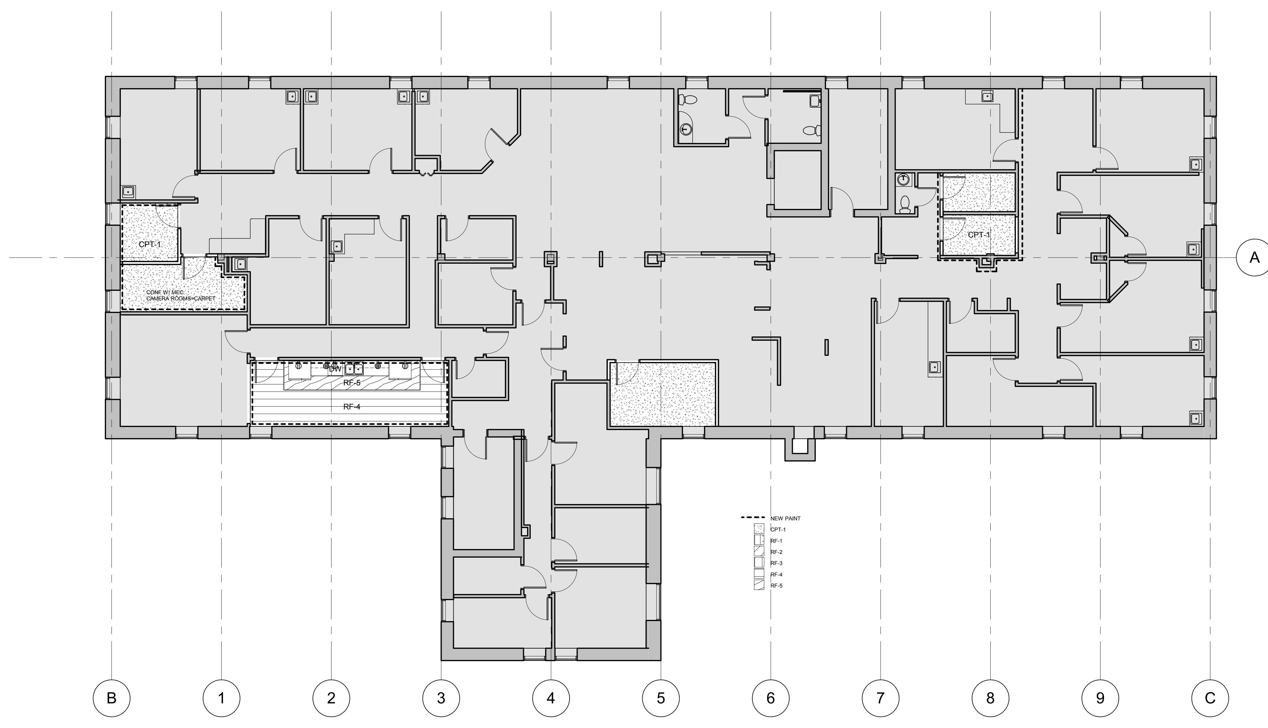
1 Level 3 - Finishes Plan 1/8" = 1'-0"
