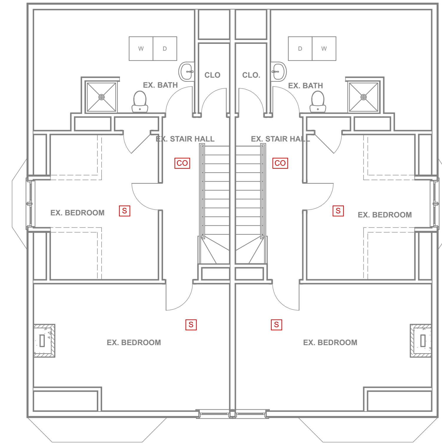
4 LIFE SAFETY THIRD FLOOR PLAN LS.1 SCALE: 3/16" = 1'-0"
