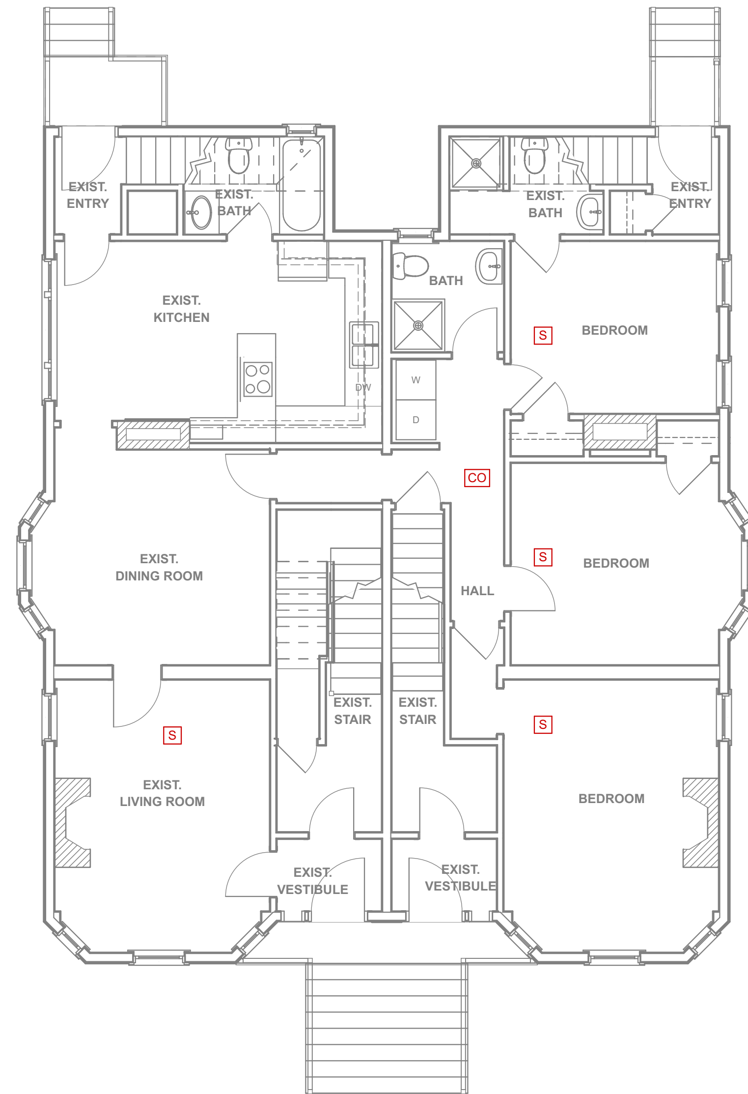
2 LIFE SAFETY FIRST FLOOR PLAN LS.1 SCALE: 3/16" = 1'-0"
