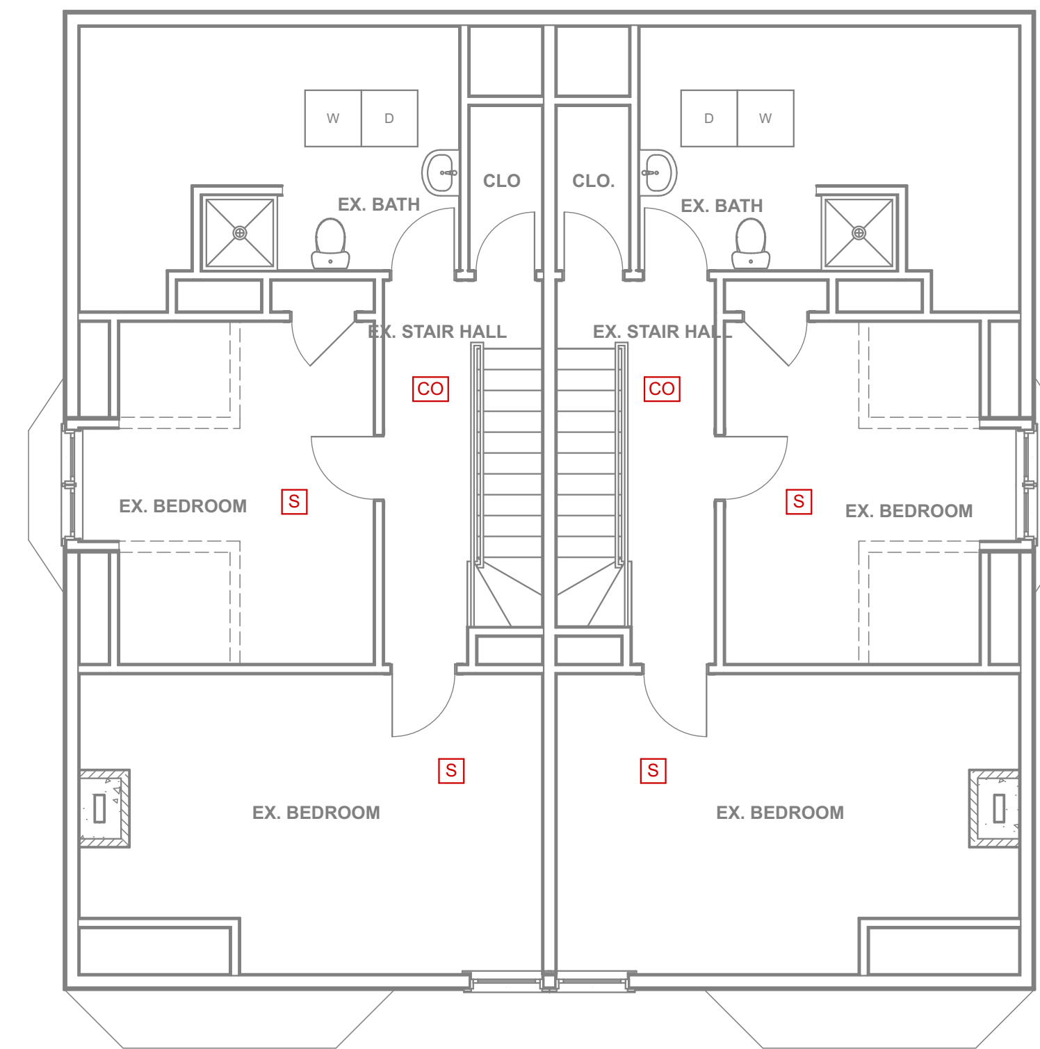
4 LIFE SAFETY THIRD FLOOR PLAN SCALE: 3/16" = 1'-0"
