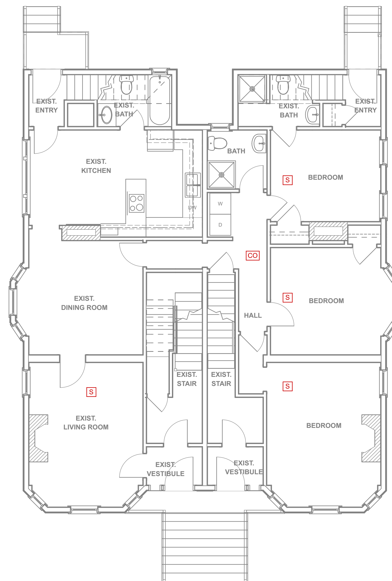
2 LIFE SAFETY FIRST FLOOR PLAN SCALE: 3/16" = 1'-0"
