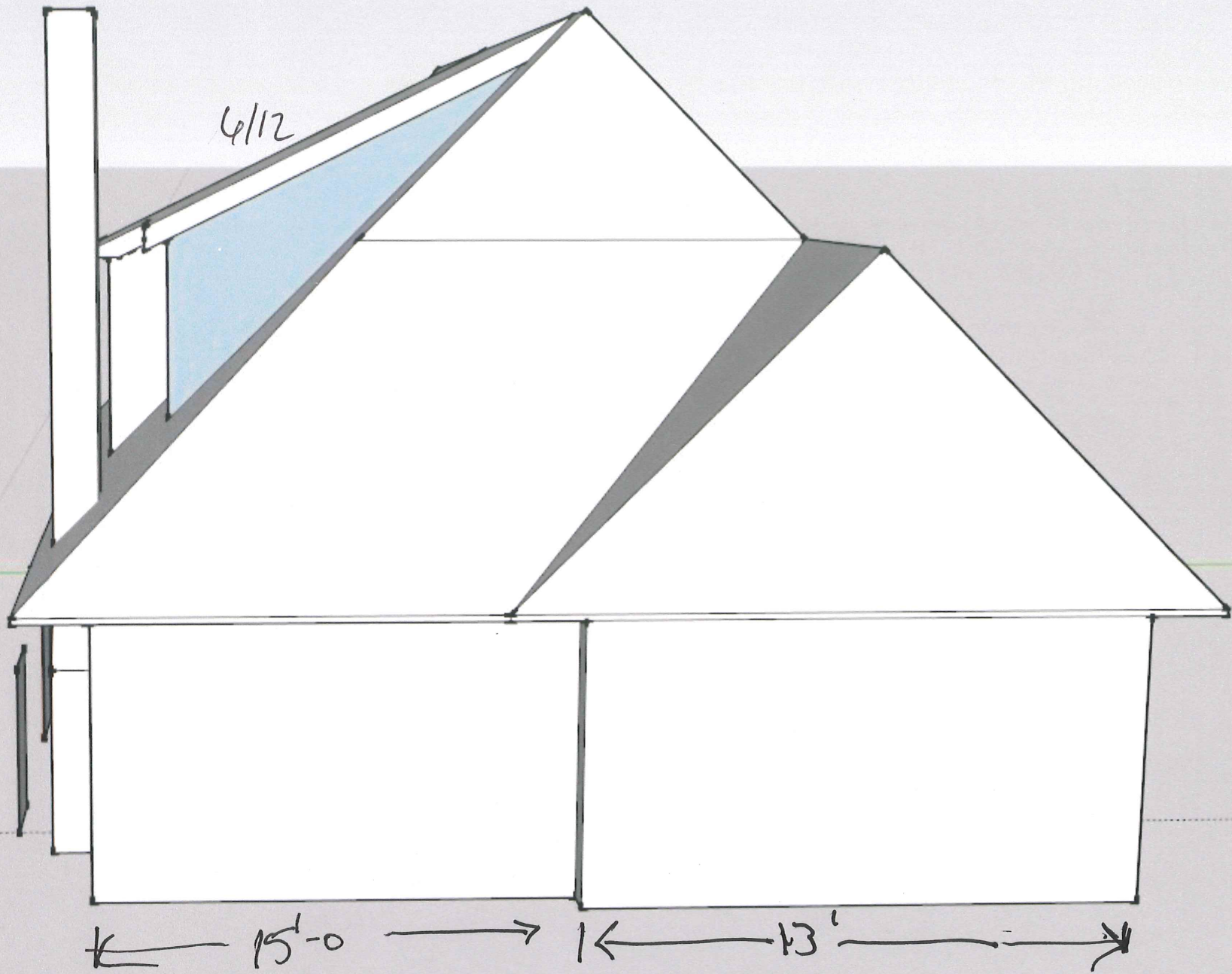
FRONT ELEVATION New
