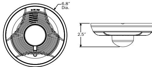
Ceiling-mount horn/strobes
