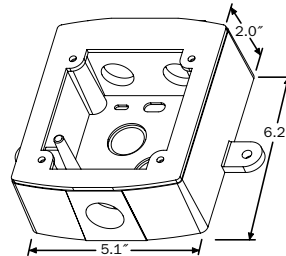
Wall weatherproof back box
