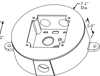
Ceiling weatherproof back box
