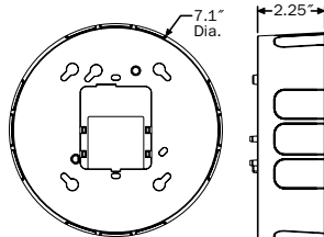
Ceiling back box skirt
