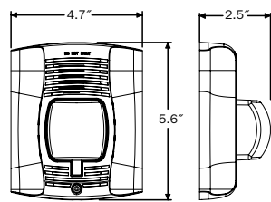
Wall-mount horn/strobes
