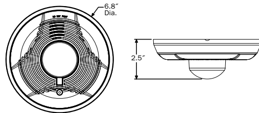
Ceiling-mount horn/strobes
