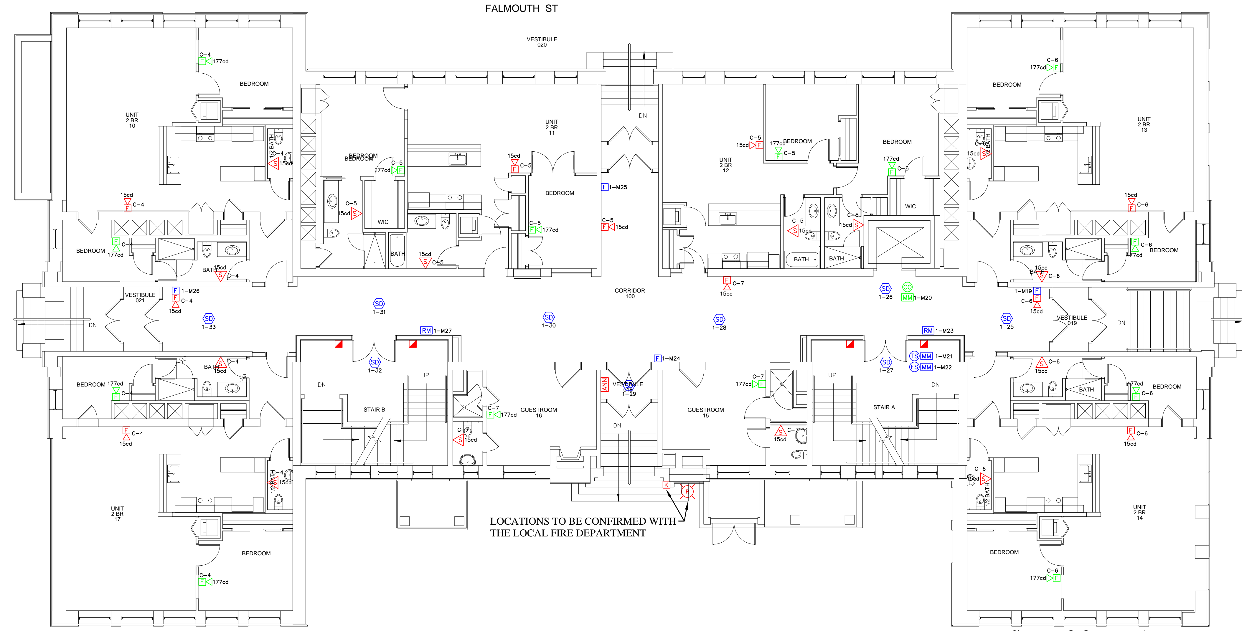
FIRST FLOOR PLAN SCALE: 1/8" = 1'-0"
