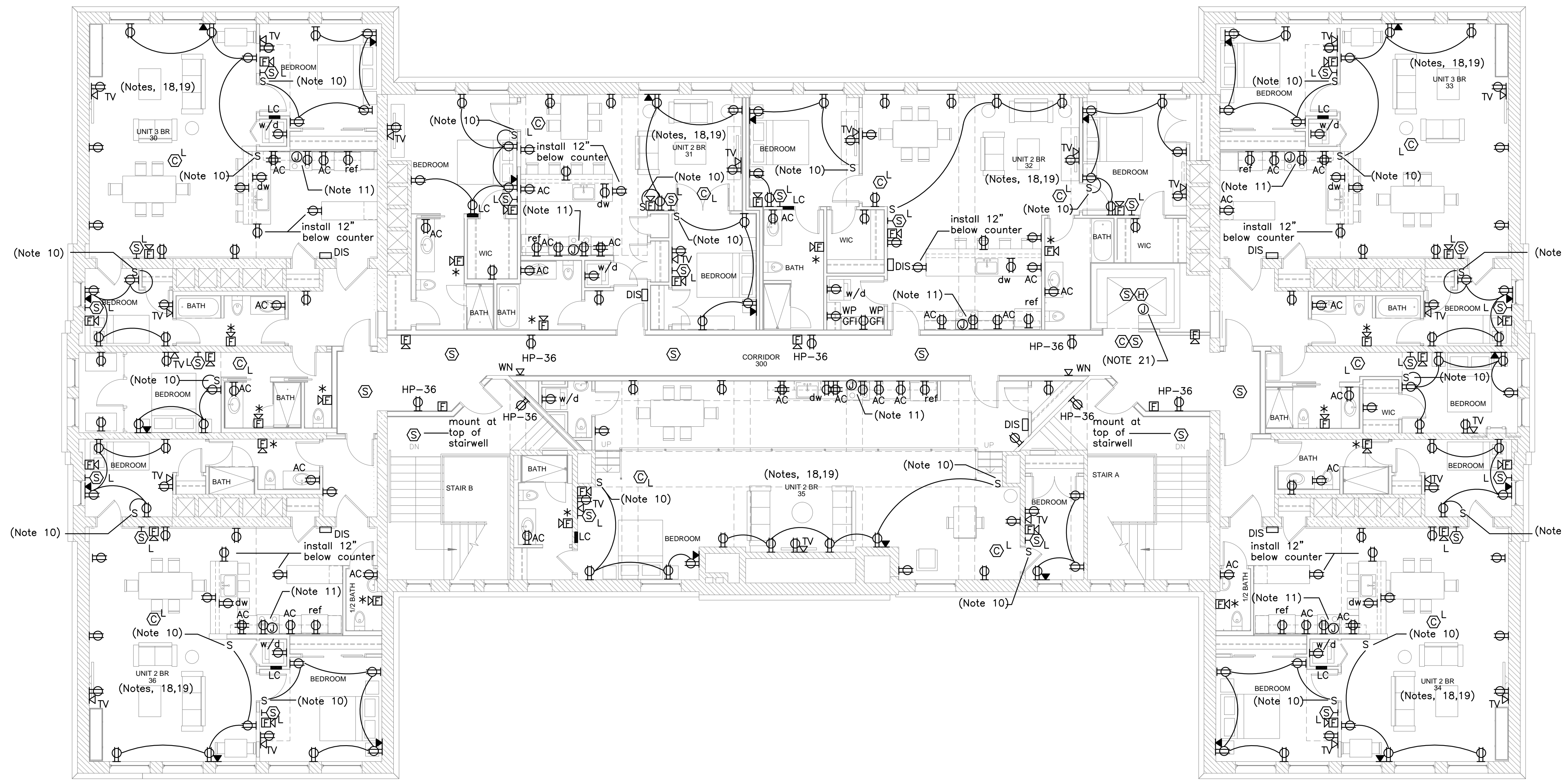
2 | THIRD FLOOR - ELECTRICAL PLAN 1/8" = 1'-0" 0 2' 4' 8'
