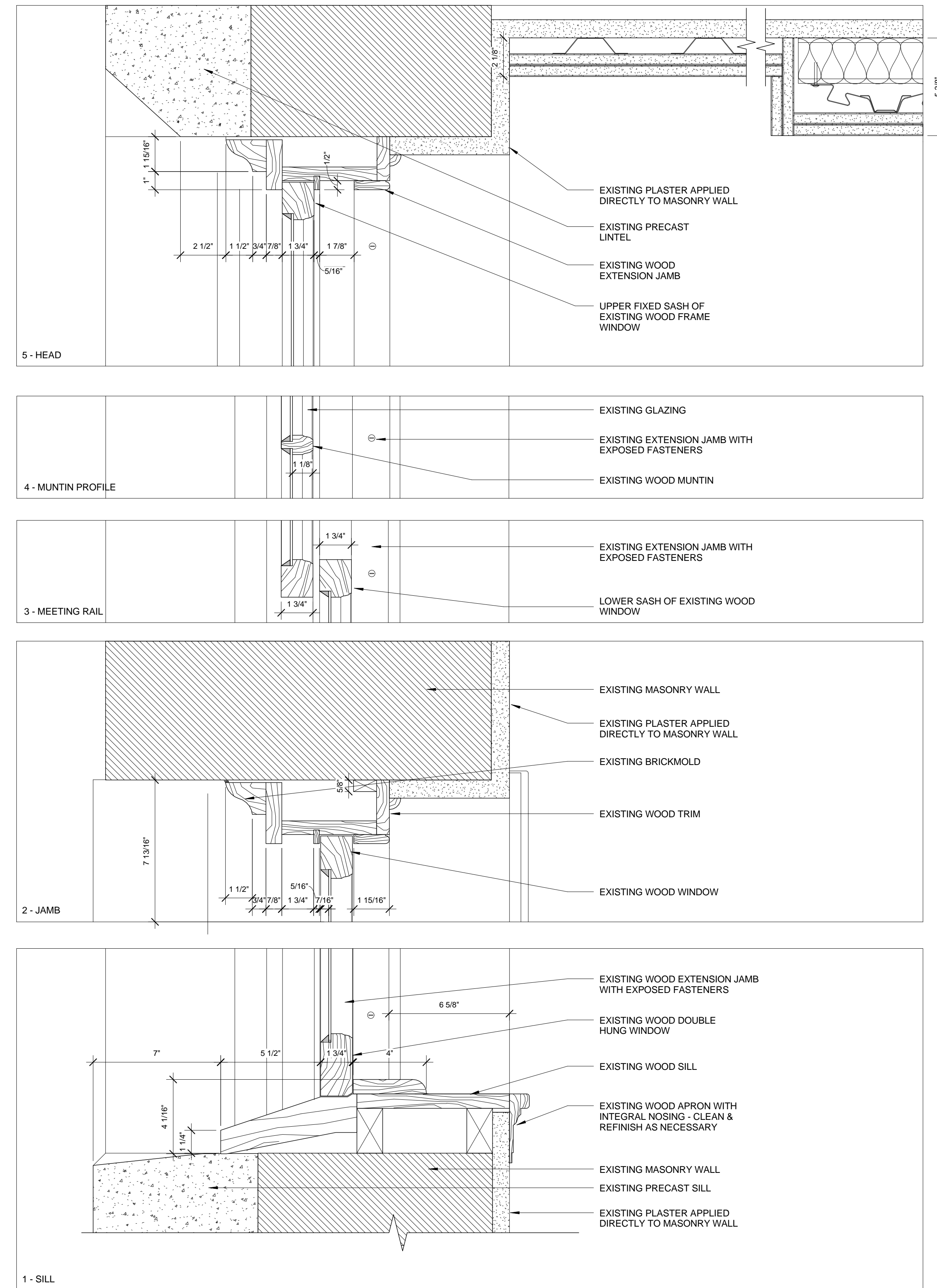
2 EXISTING WOOD WINDOW SECTION - TO BE REMOVED 3" = 1'-0"
