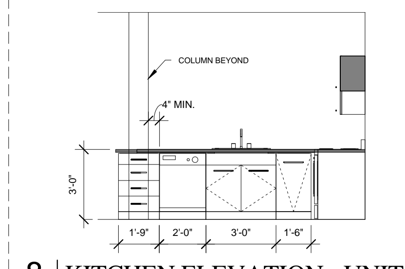
8 | KITCHEN ELEVATION - UNIT 02 1/4" = 1'-0"
