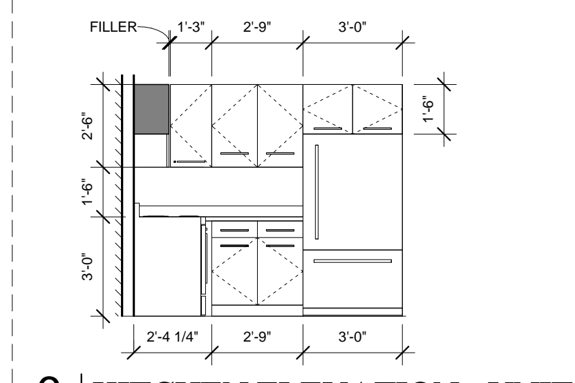
6 | KITCHEN ELEVATION - UNIT 02 1/4" = 1'-0"
