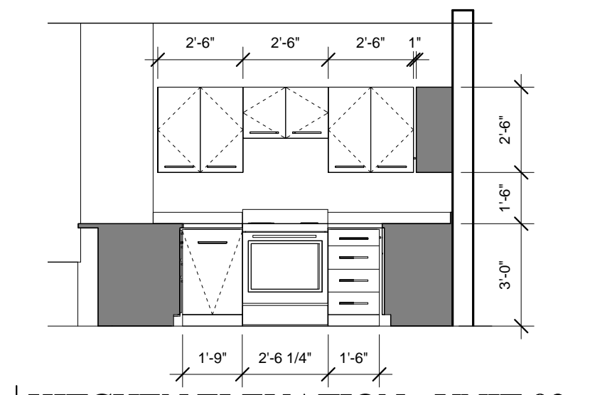
7 | KITCHEN ELEVATION - UNIT 02 1/4" = 1'-0"
