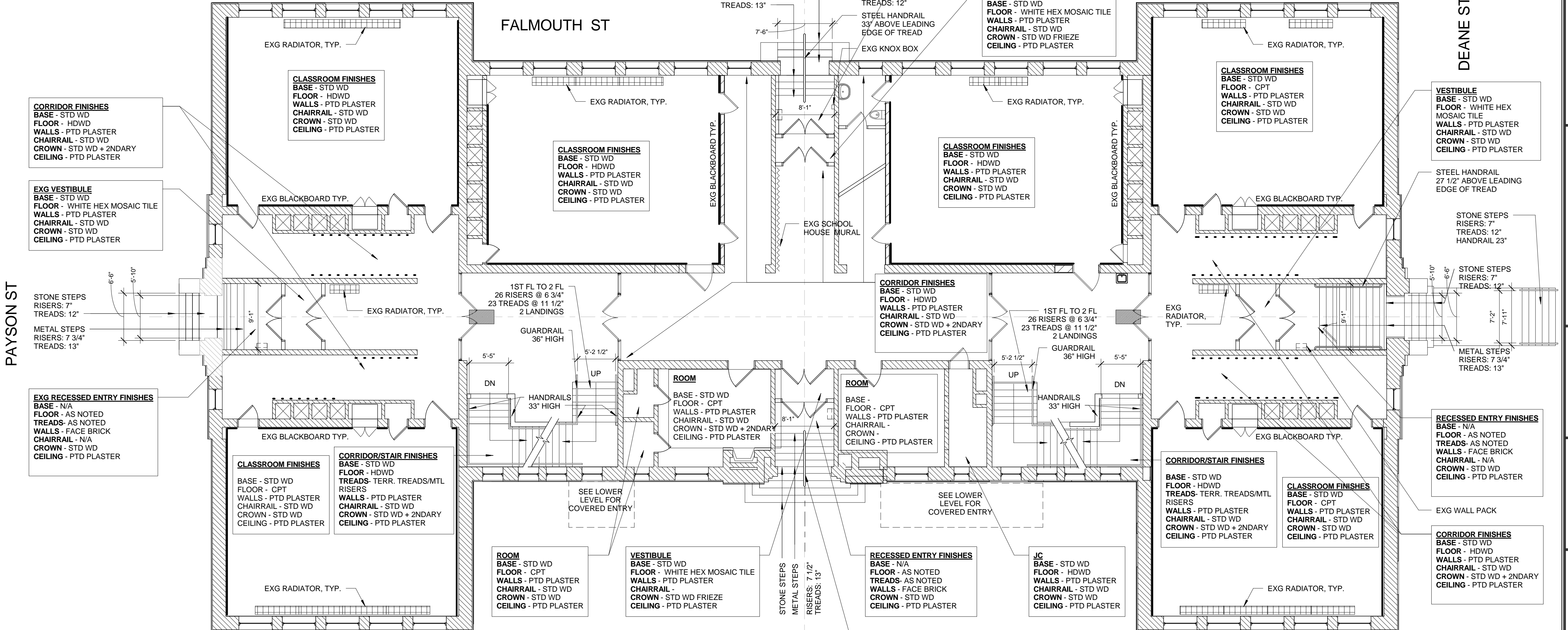
1 | FIRST FLOOR - EXISTING PLAN
