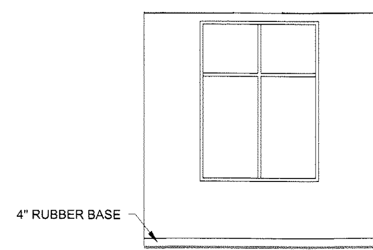
A2 OFFICE 2 - EAST 1/4" = 1'-0"
