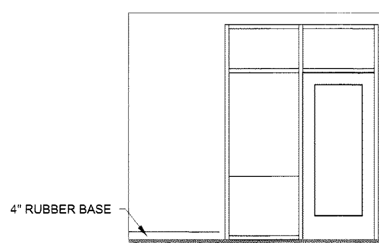
A3 OFFICE 2 - SOUTH 1/4" = 1'-0"
