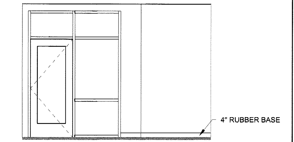
D1 OFFICE 1 - NORTH 1/4" = 1'-0"
