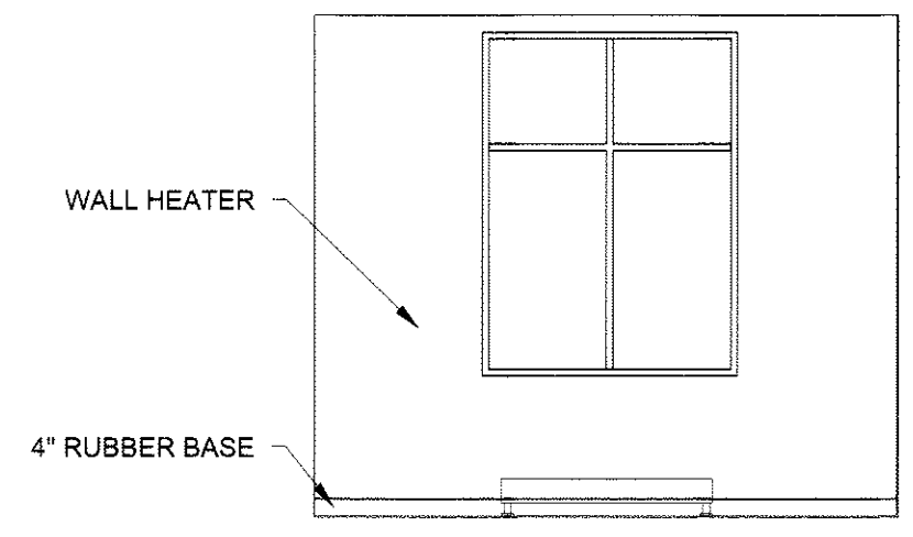
C1 OFFICE 4 - NORTH 1/4" = 1'-0"
