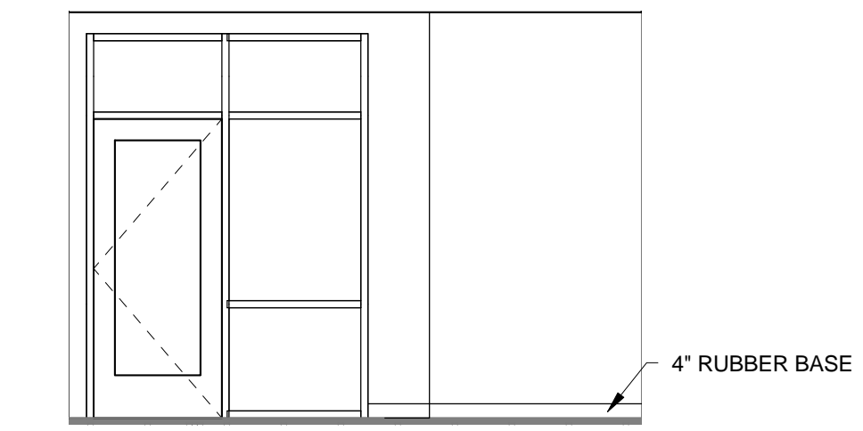
D1 OFFICE 1 - NORTH 1/4" = 1'-0"
