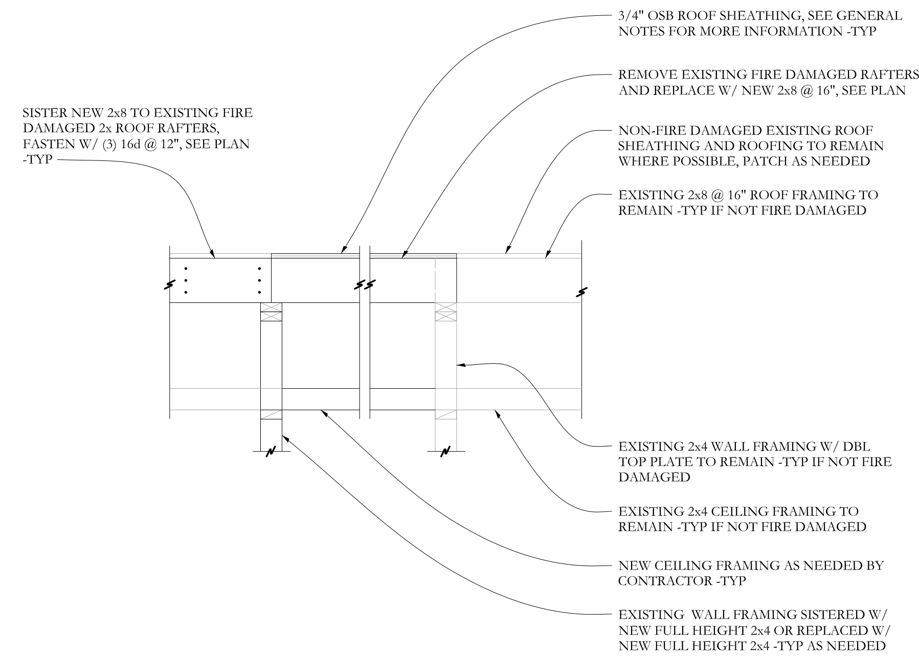
SECTION D (S-2.1) 3/4"=1'-0"
