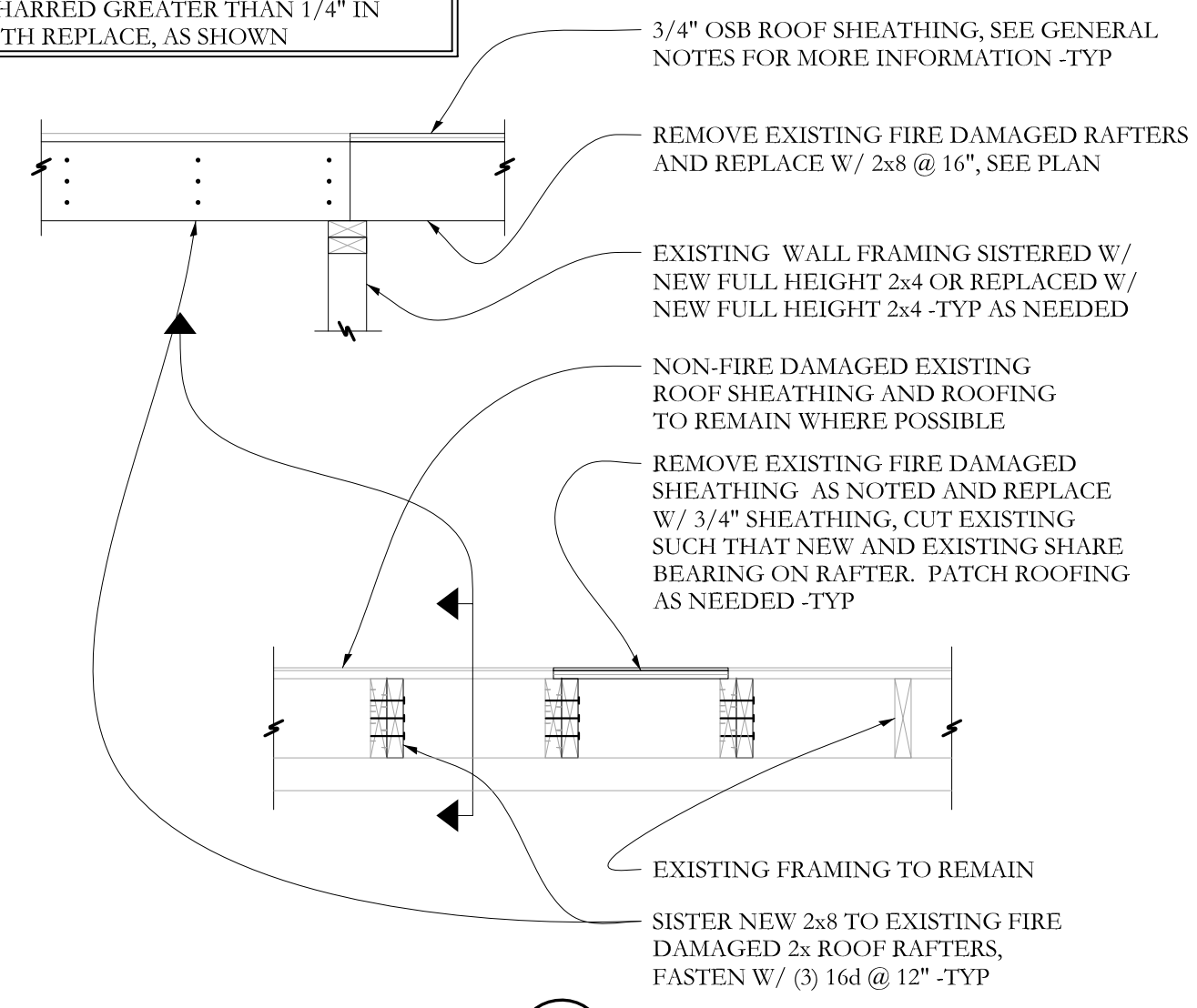
SECTION B (S-2.1) 3/4"=1'-0"
