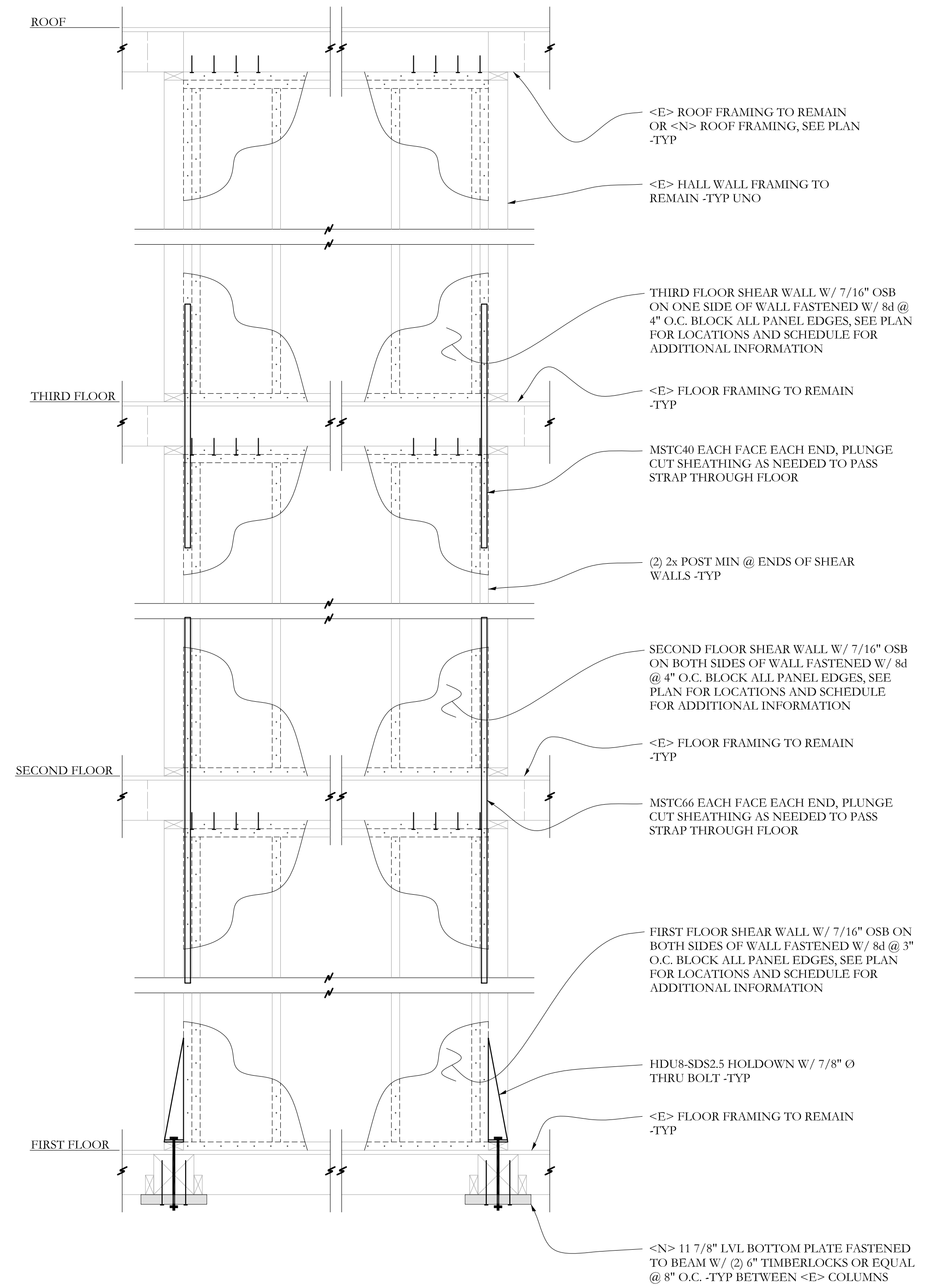
SECTION C (S-2.1) 3/4"=1'-0"
