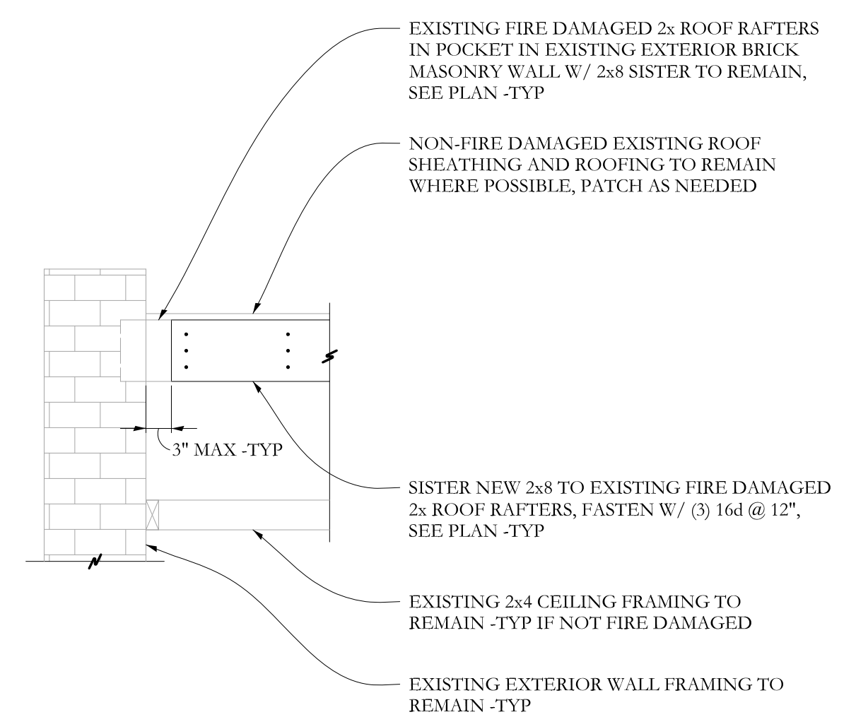
SECTION E (S-2.1) 3/4"=1'-0"
