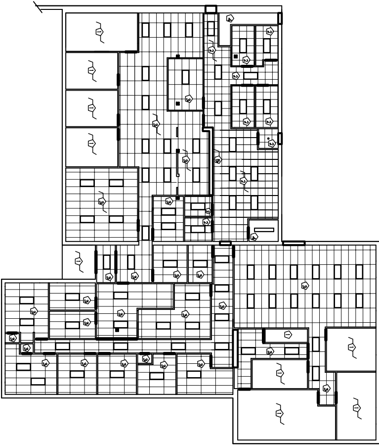
1 FIRST FLOOR REFLECTED CEILING PLAN SCALE: 1/8" = 1'-0"
