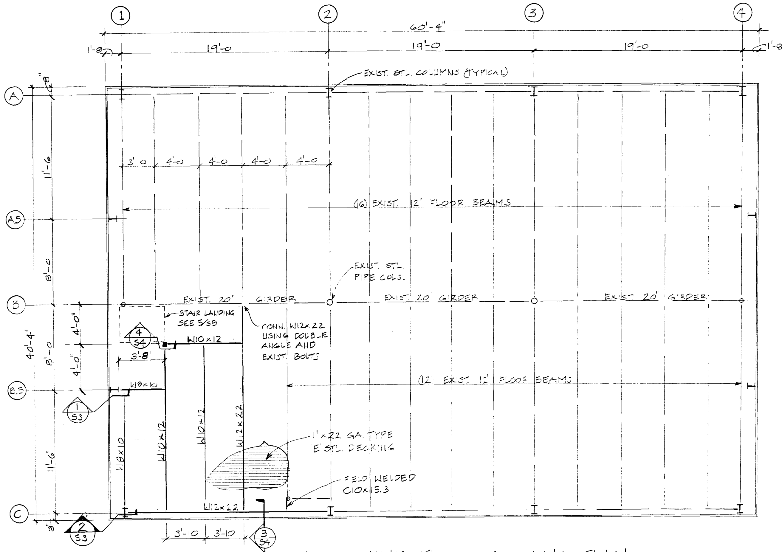
MEZZANINE FLOOR FRAMING PLAN
