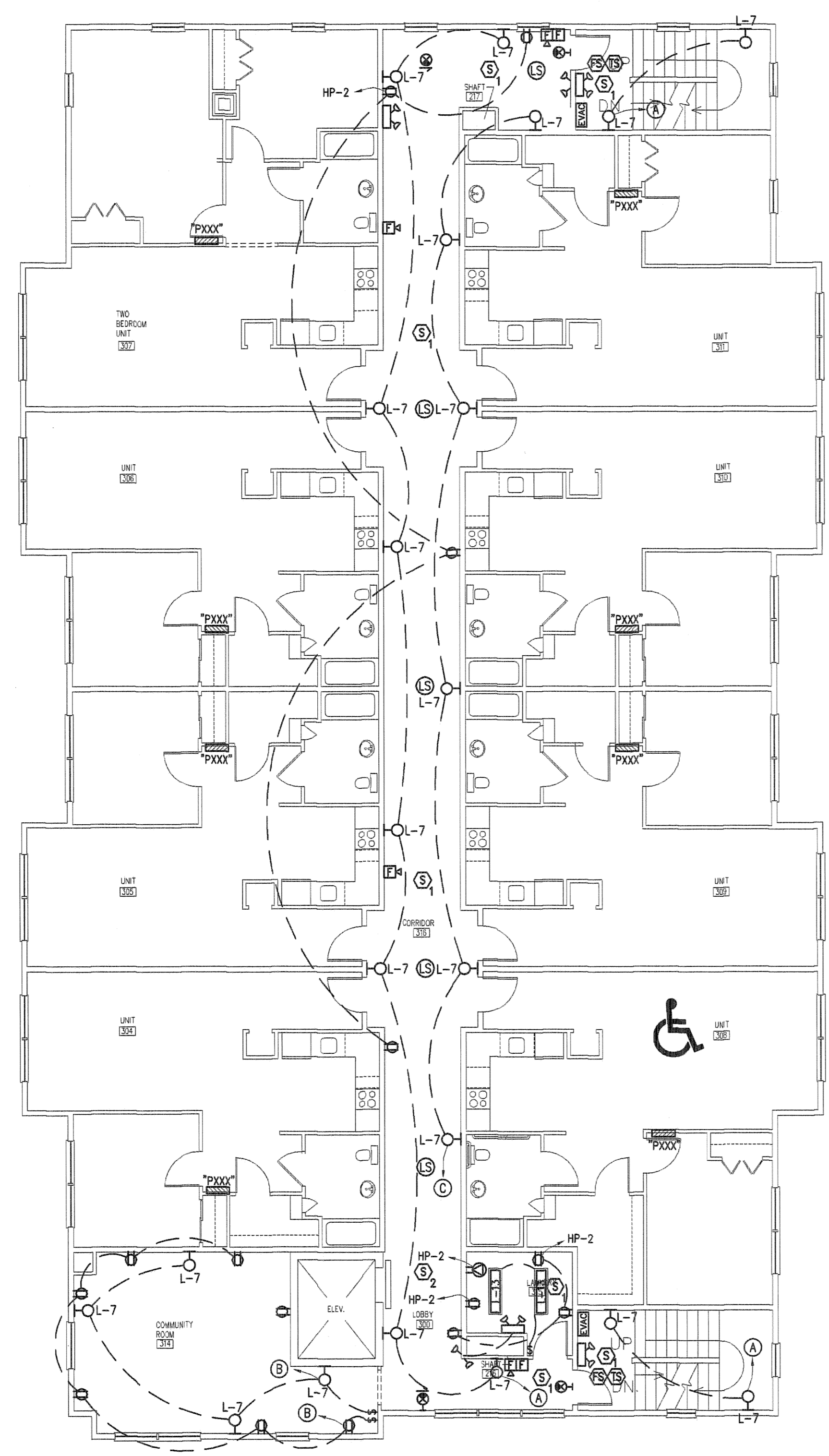
3 THIRD FLOOR PLAN A.1 SCALE: 1/8" = 1'-0"
