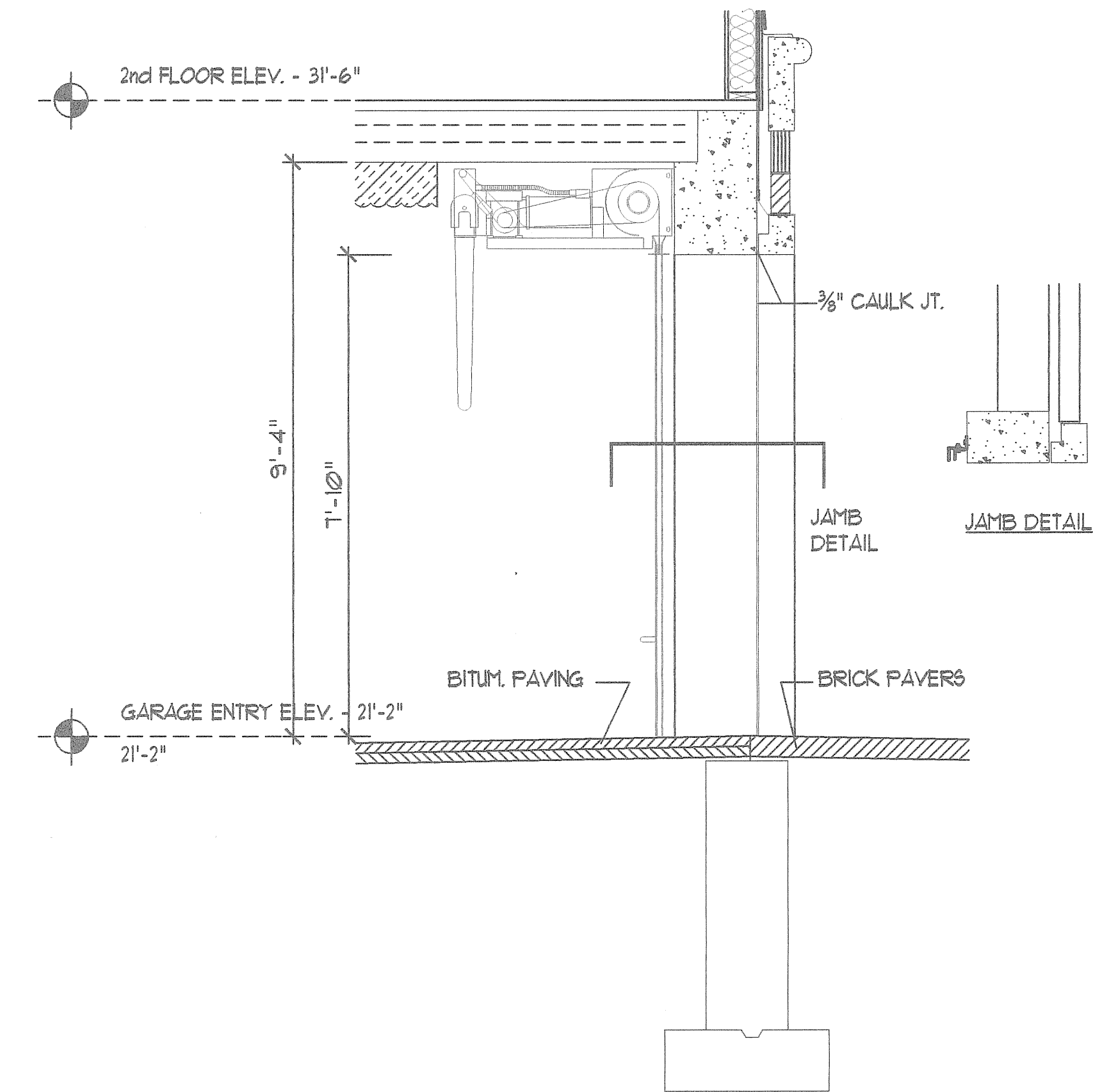
1 SECTION AT GARAGE DOOR A11a SCALE 1/2" = 1'-0"
