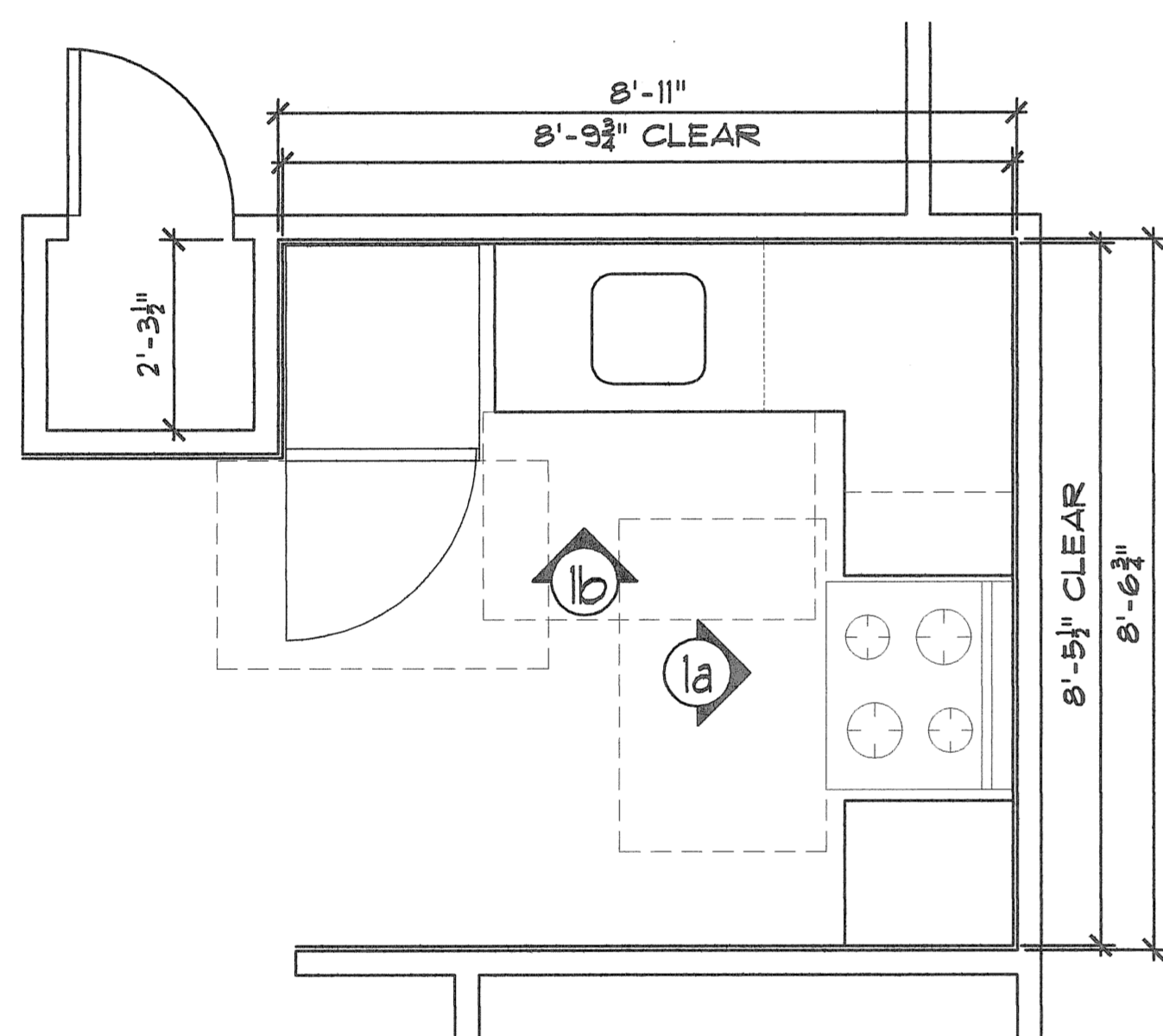
1 TYPICAL KITCHEN FLOOR PLAN SCALE: 1/2" = 1'-0"
