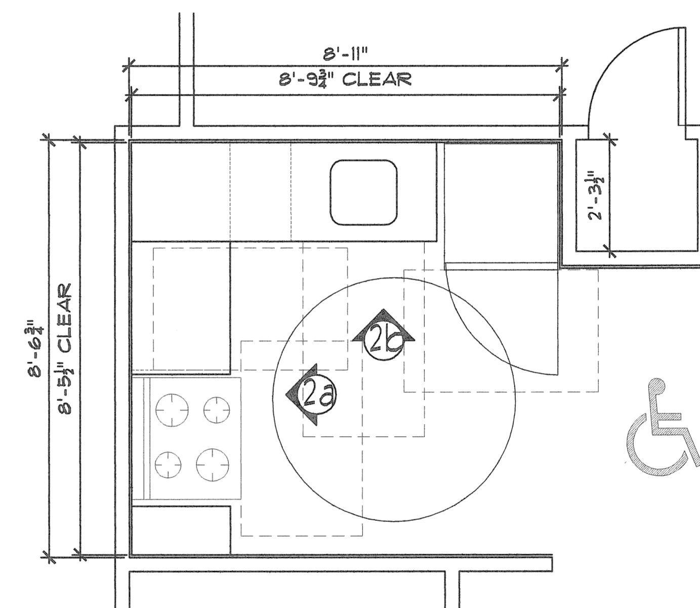
2 TYPICAL ACCESSIBLE KITCHEN FLOOR PLAN SCALE: 1/2" = 1'-0"
