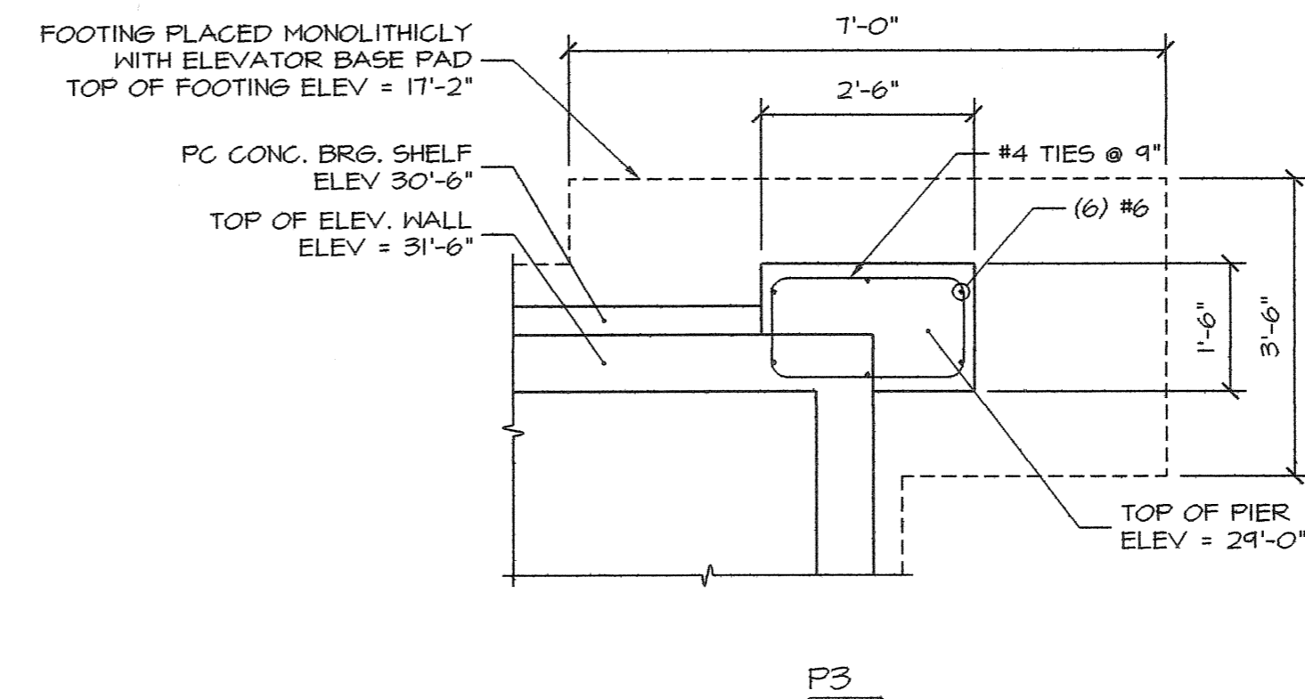
PIER DETAILS 1/2"=1'-0"
