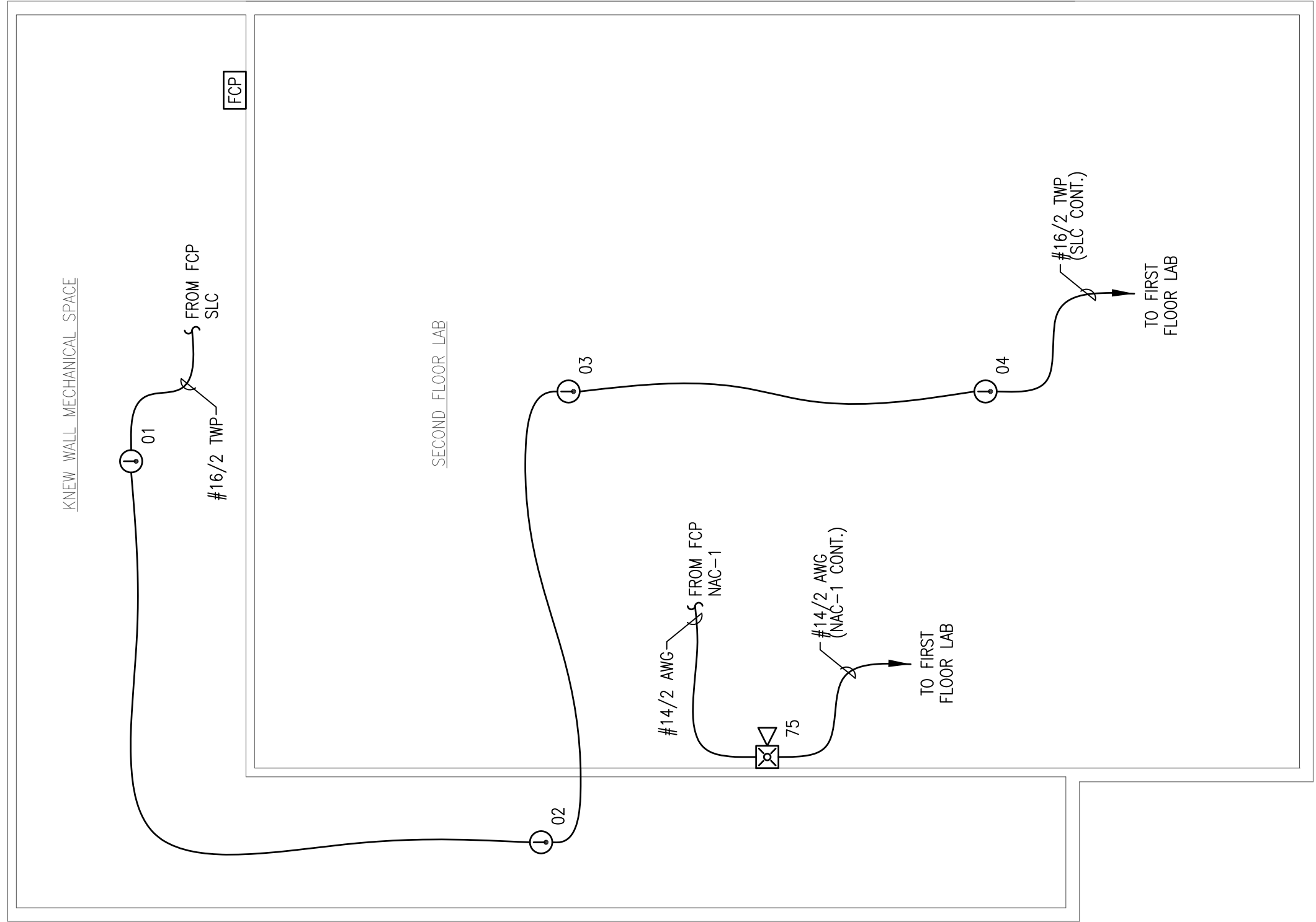
SECOND FLOOR FIRE ALARM PLAN SCALE: 1/8"=1'-0"
