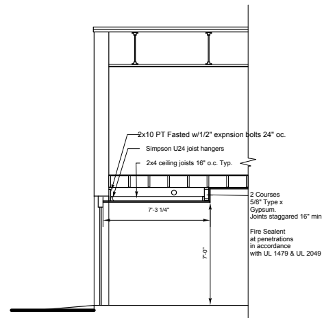
Section EE Proposed SCALE: 1/4" = 1'-0"
