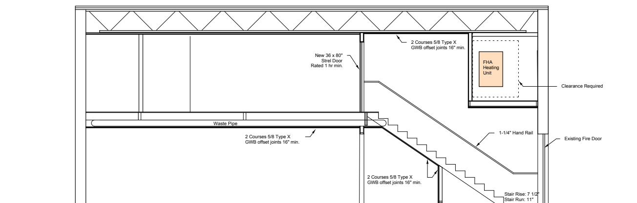
Proposed Section DD SCALE: 1/4" = 1'-0"
