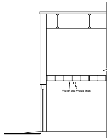
Section EE Existing SCALE: 1/4" = 1'-0"
