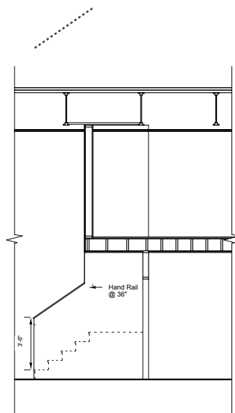
Section CC Proposed SCALE: 1/4" = 1'-0"
