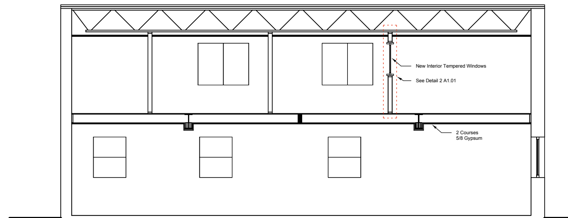
Section BB Proposed SCALE: 1/4" = 1'-0"
