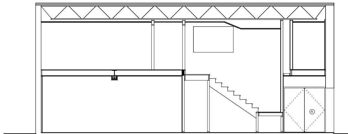
Section AA Proposed SCALE: 1/4" = 1'-0"
