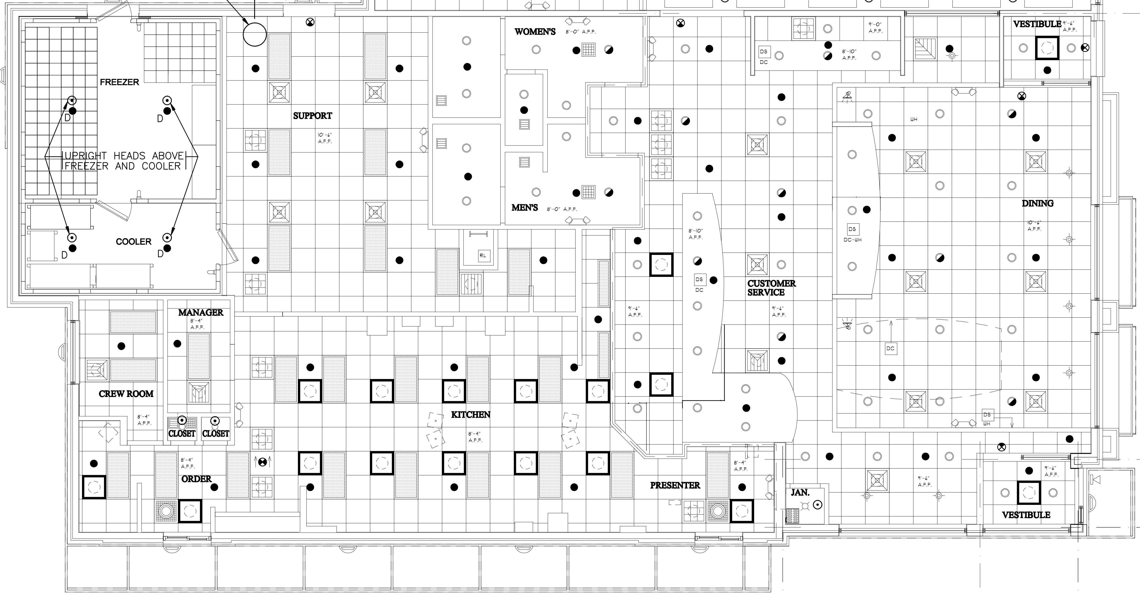
SPRINKLER SCOPE PLAN SCALE: 1/4"=1'-0"
