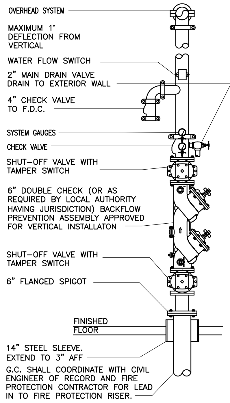
DETAIL-FIRE RISER NO SCALE
