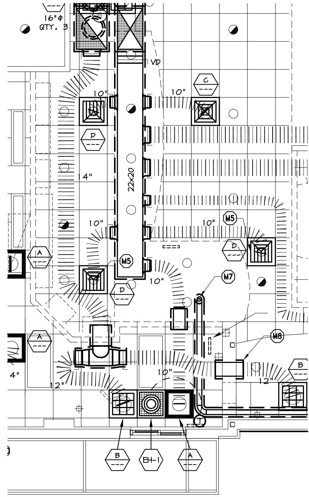
MECHANICAL PLAN 1/4" = 1'-0"
