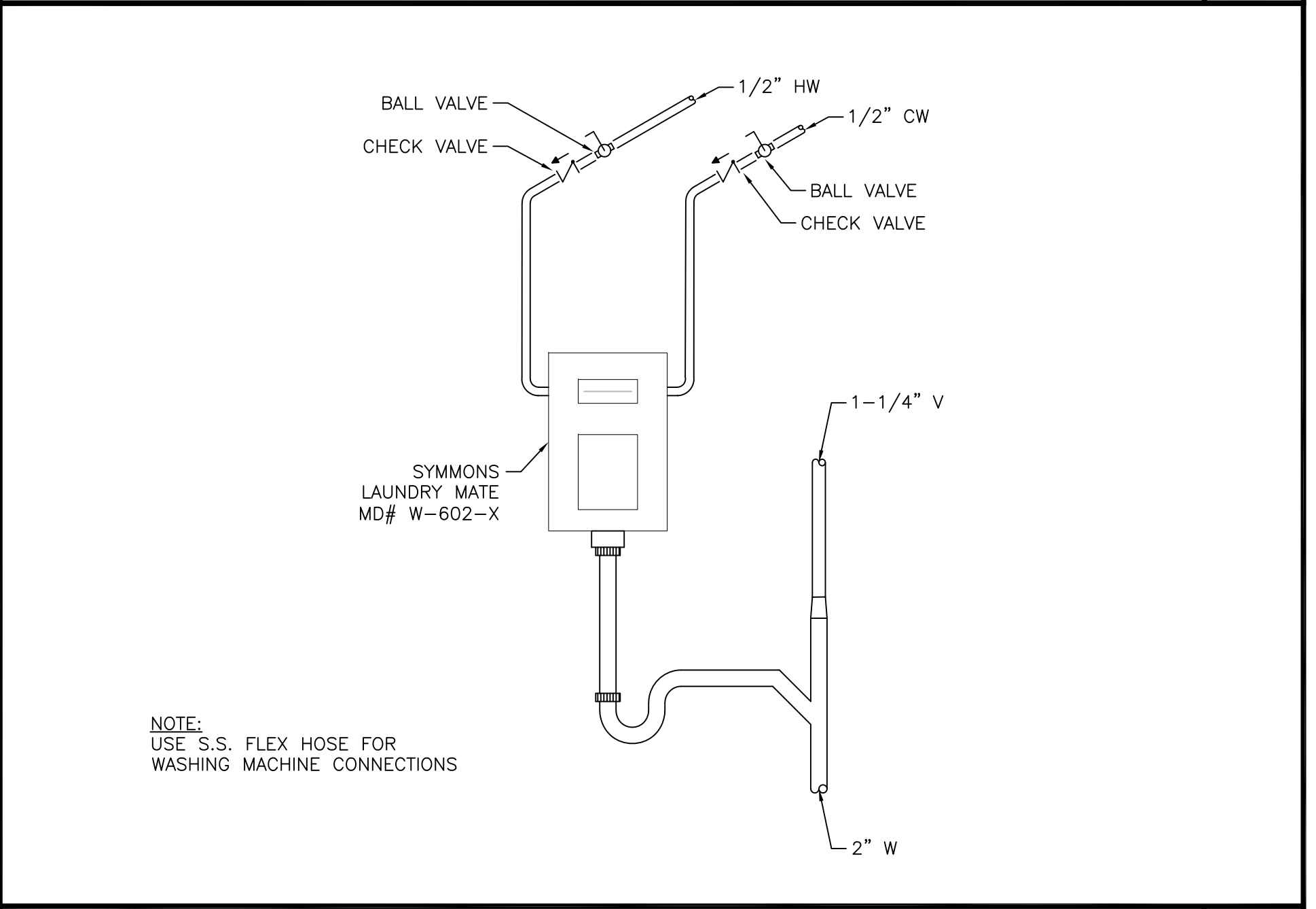
DOMESTIC WASHING MACHINE DETAIL
