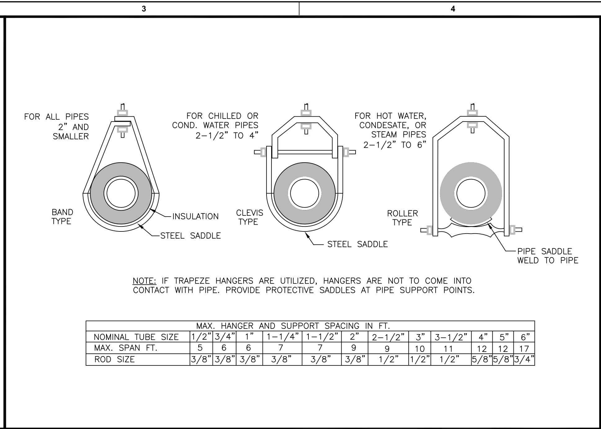
PIPE HANGER STANDARDS DETAIL
