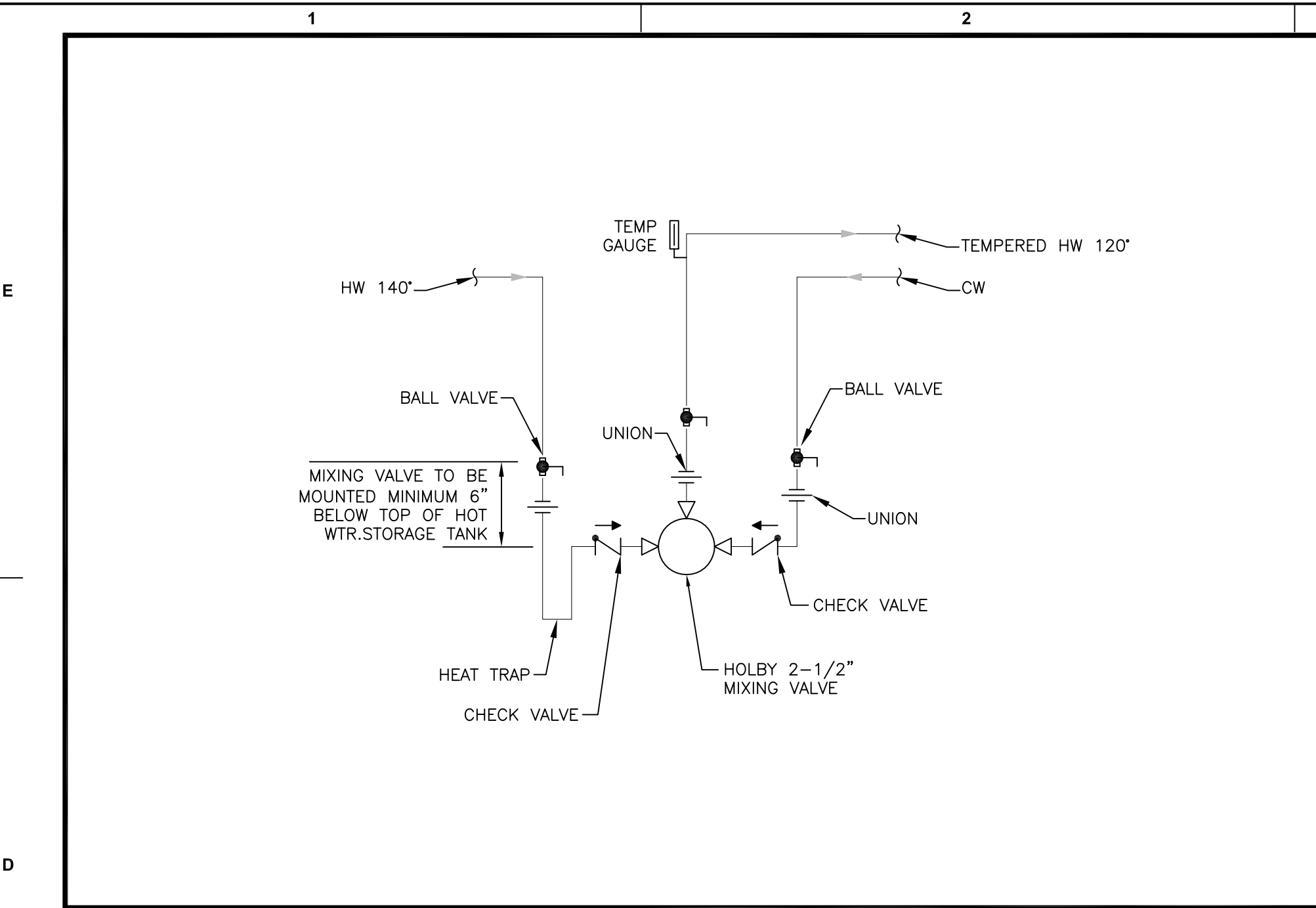
MIXING VALVE DETAIL
