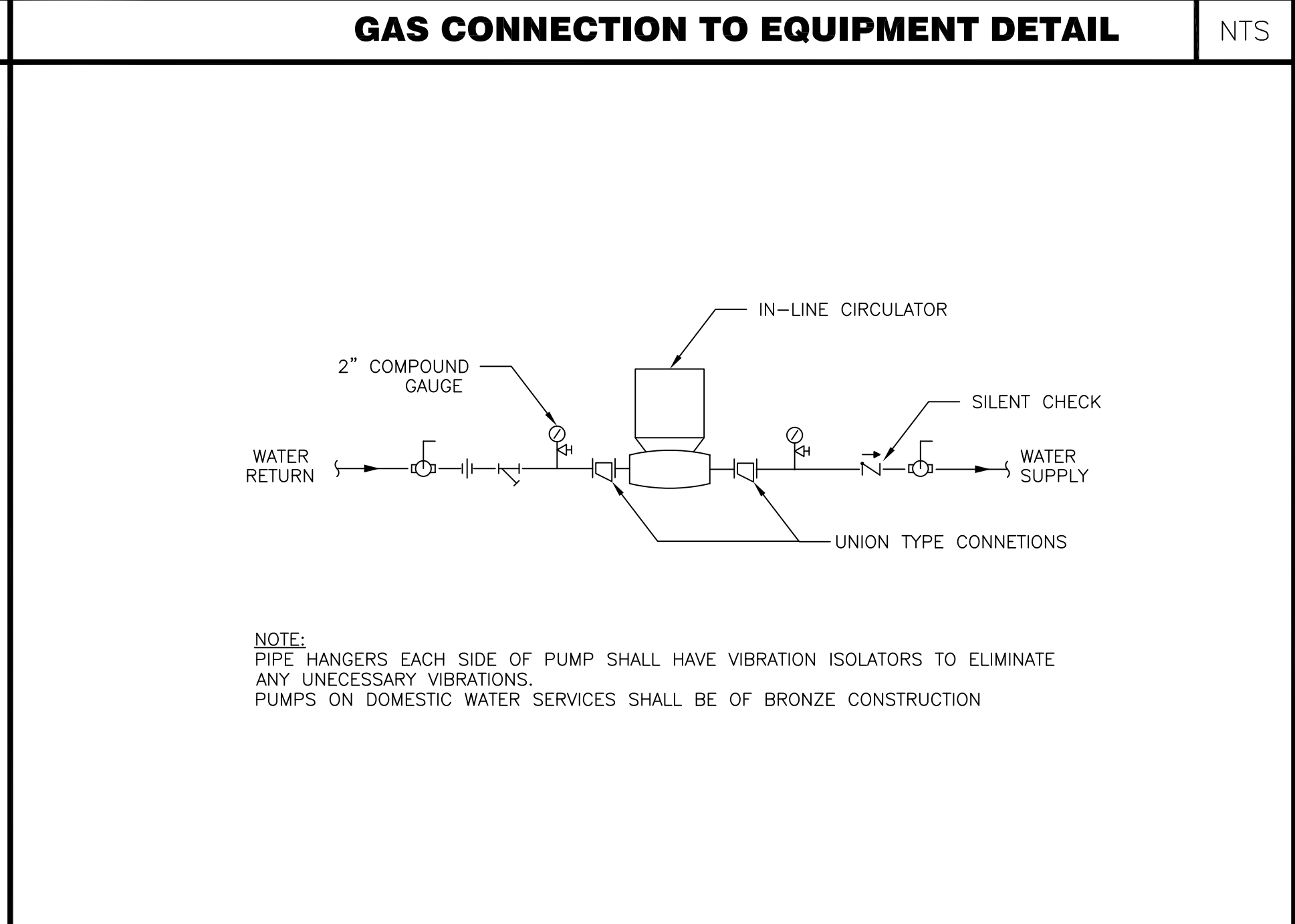
IN-LINE CIRCULATOR DETAIL
