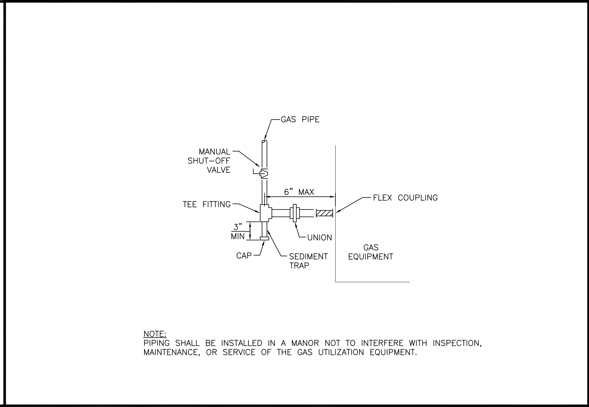
GAS CONNECTION TO EQUIPMENT DETAIL
