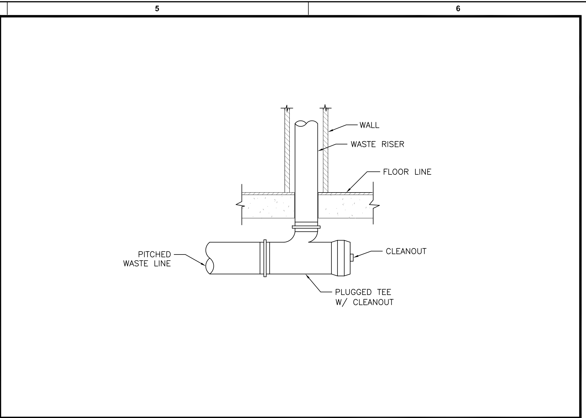
WASTE PIPE CLEANOUT DETAIL
