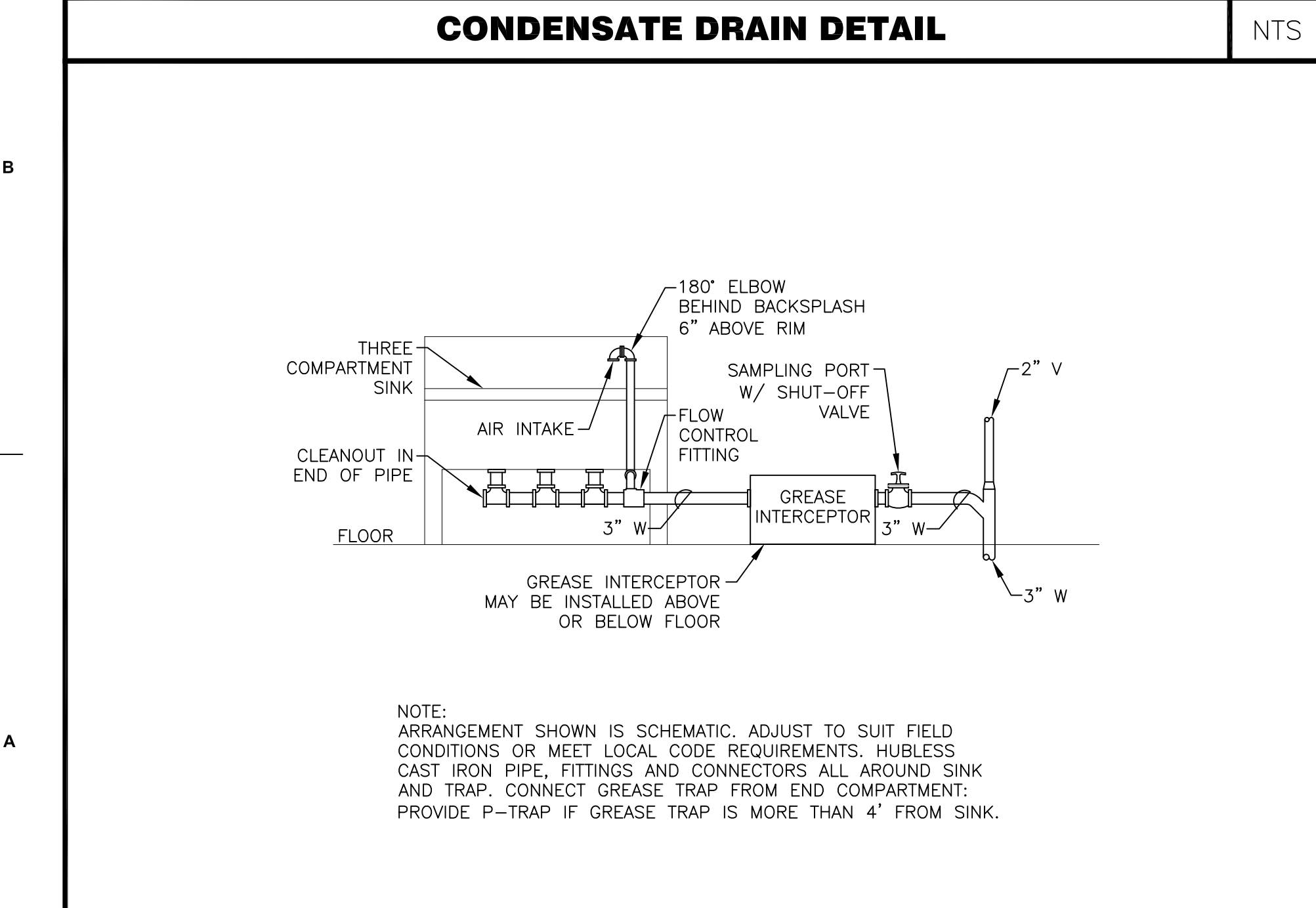
GREASE INTERCEPTOR DETAIL
