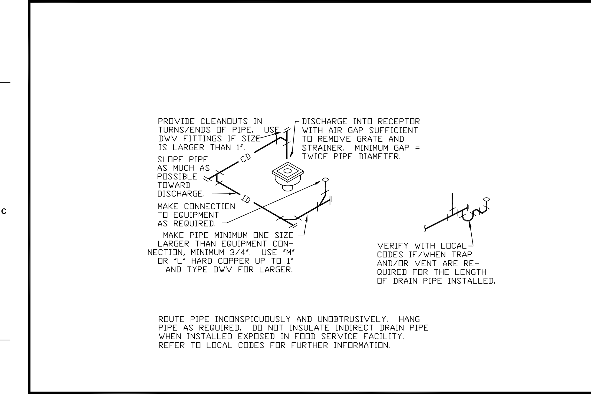
CONDENSATE DRAIN DETAIL
