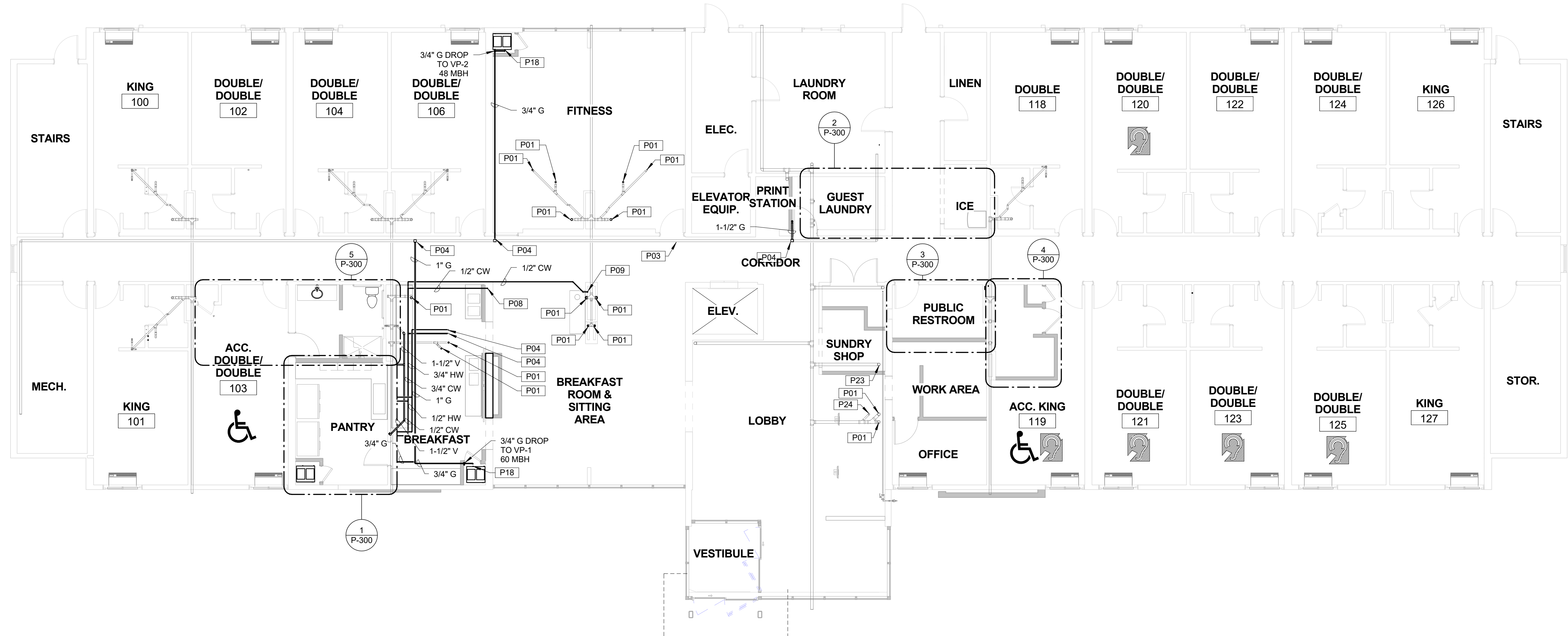
① FIRST FLOOR PLAN - Plumbing 1/8" = 1'-0"
