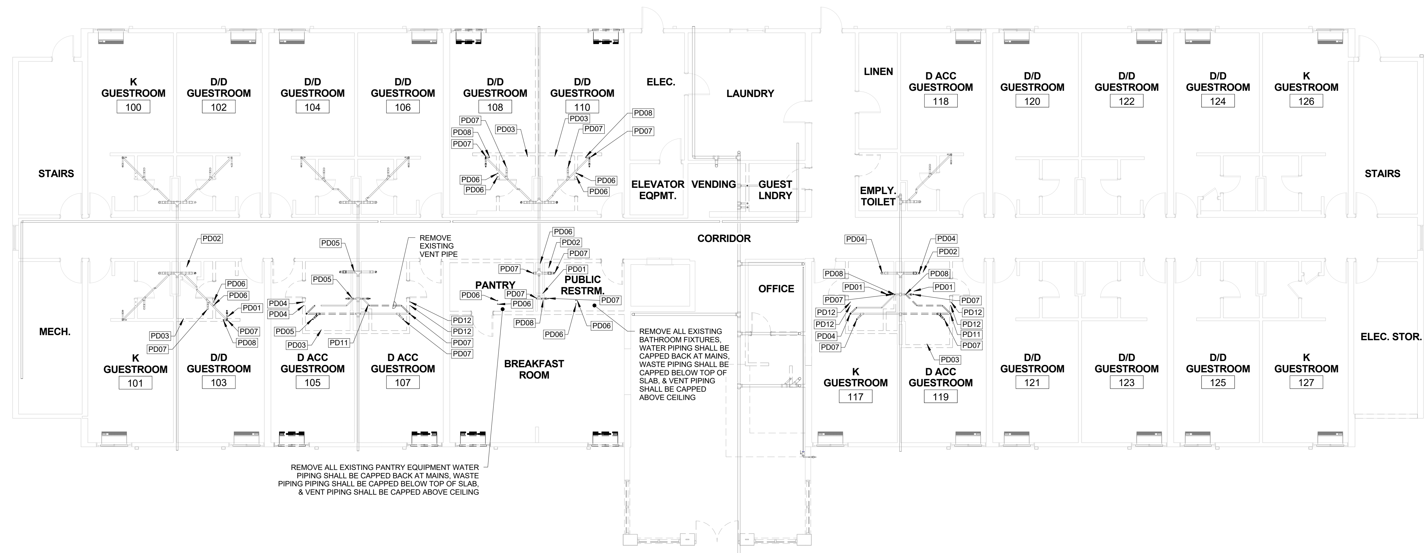
FIRST FLOOR DEMOLITION PLAN - Plumbing 1/8" = 1'-0"
