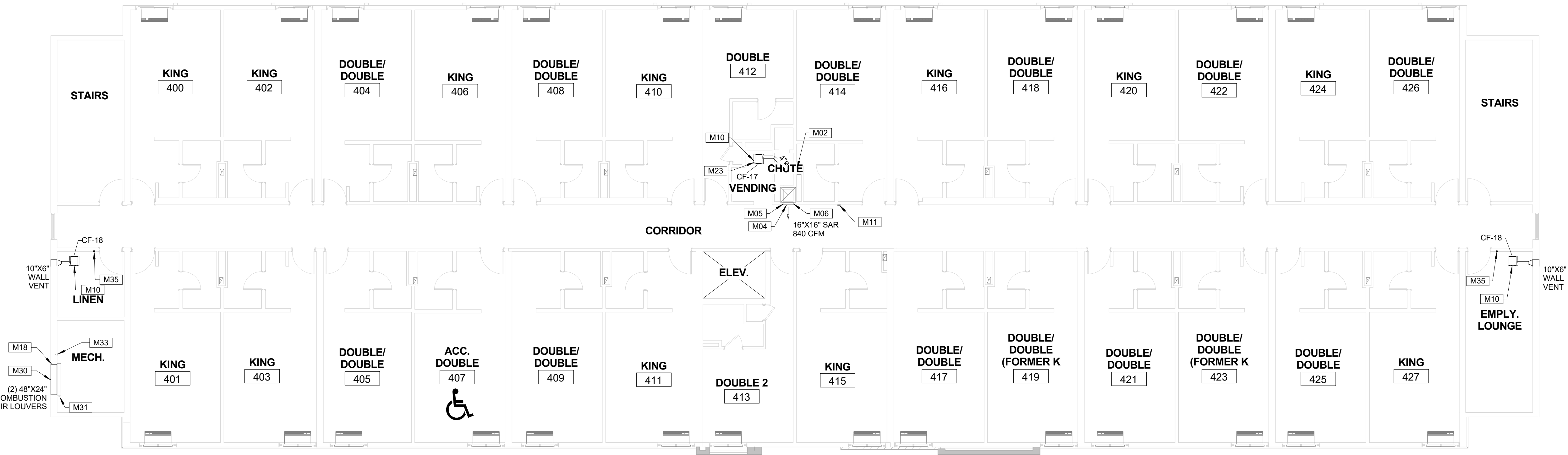
1 FOURTH FLOOR PLAN 1/8" = 1'-0"
