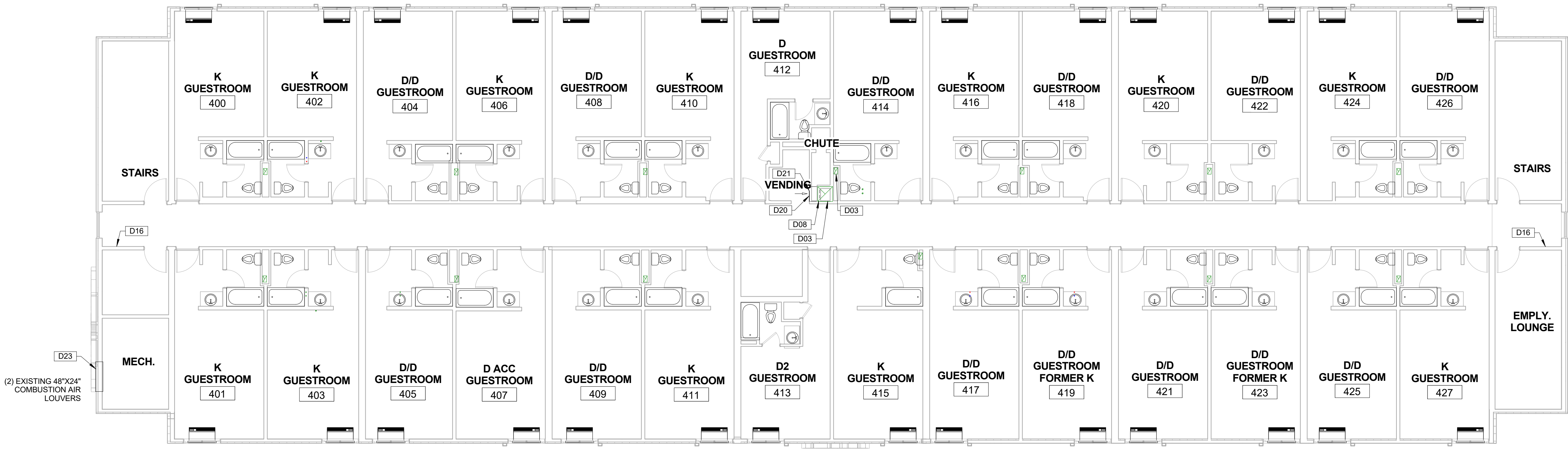
① FOURTH FLOOR DEMOLITION PLAN 1/8" = 1'-0"
