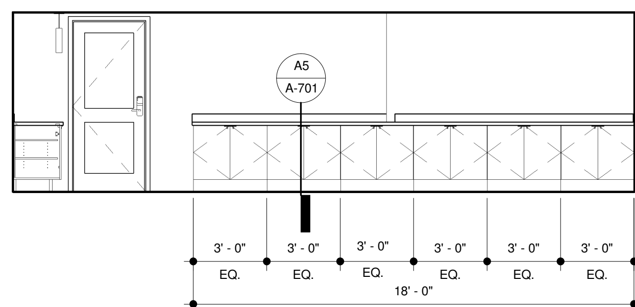
E1 INT ELEV - BREAKFAST PANTRY 1/4" = 1'-0"
