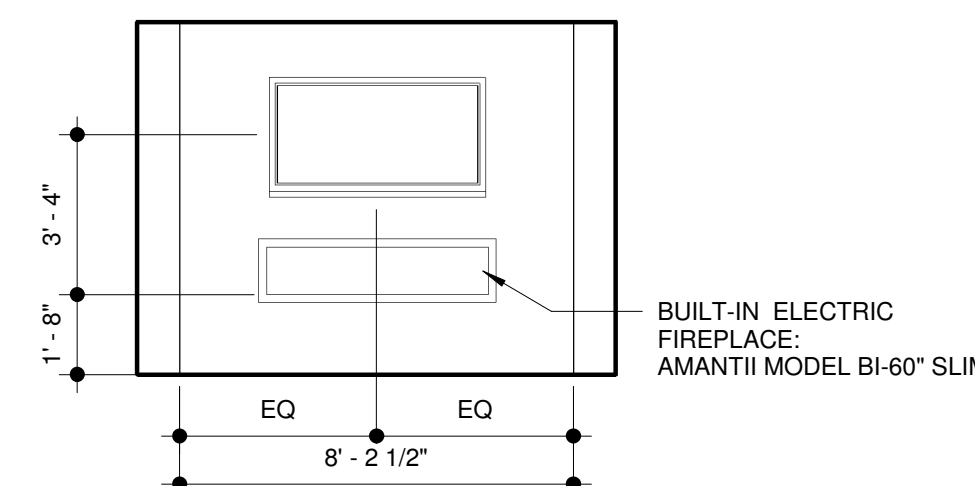
C4 FIRE PLACE ELEVATION 1/4" = 1'-0"
