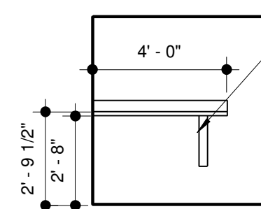
C2 FOLDING COUNTER ELEVATION 1/4" = 1'-0"
