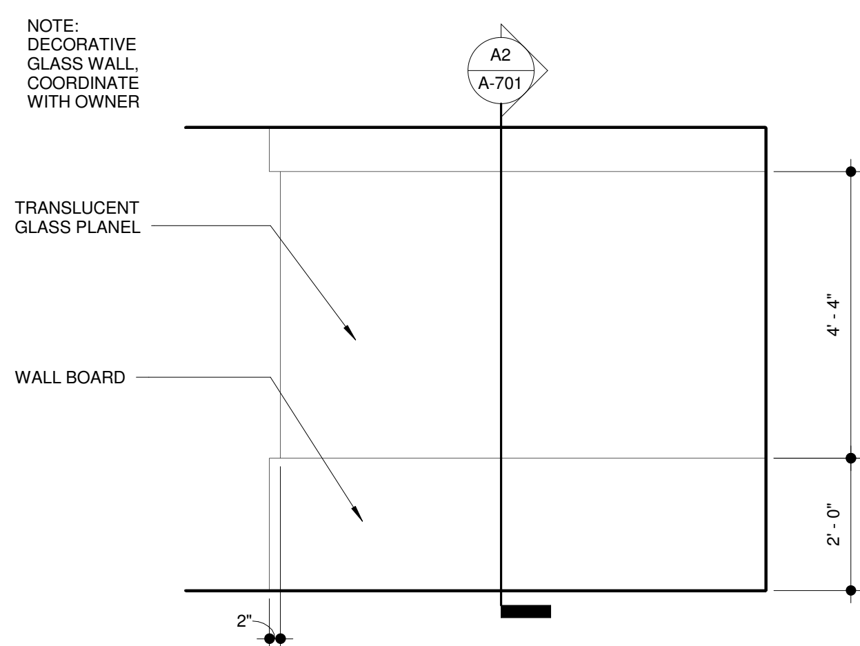
A1 INT ELEV - GLASS PARTITION WALL 1/2" = 1'-0"
