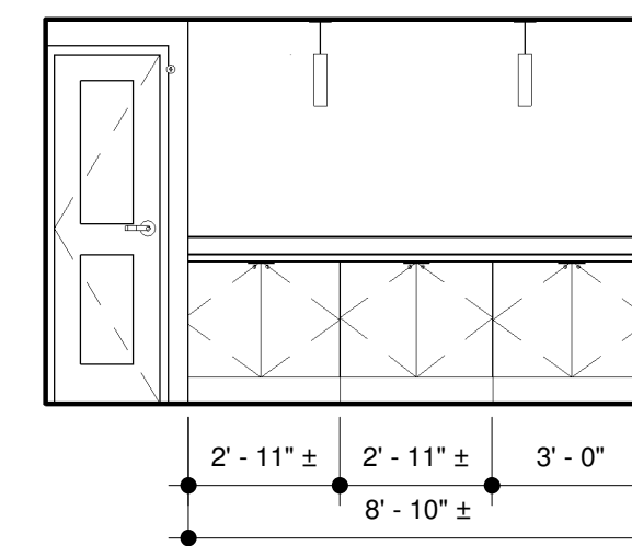
E5 INT ELEV - BREAKFAST PANTRY 1/4" = 1'-0"
