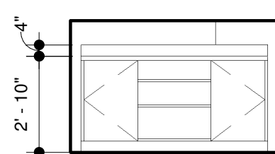
C1 COFFEE STATION ELEVATION 1/4" = 1'-0"
