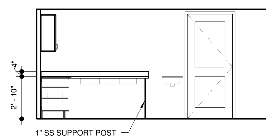
D4 INT. ELEV - KITCHEN - 3 1/4" = 1'-0"
