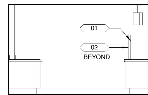
E2 INT ELEV - BREAKFAST PANTRY 1/4" = 1'-0"
