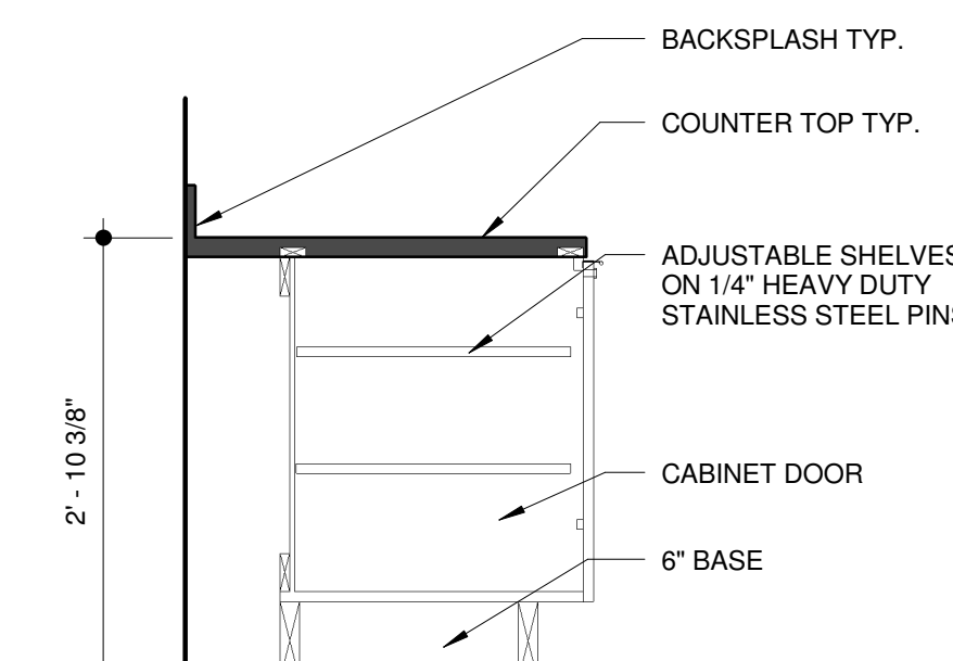
A5 MILLWORK SECTION 3/4" = 1'-0"
