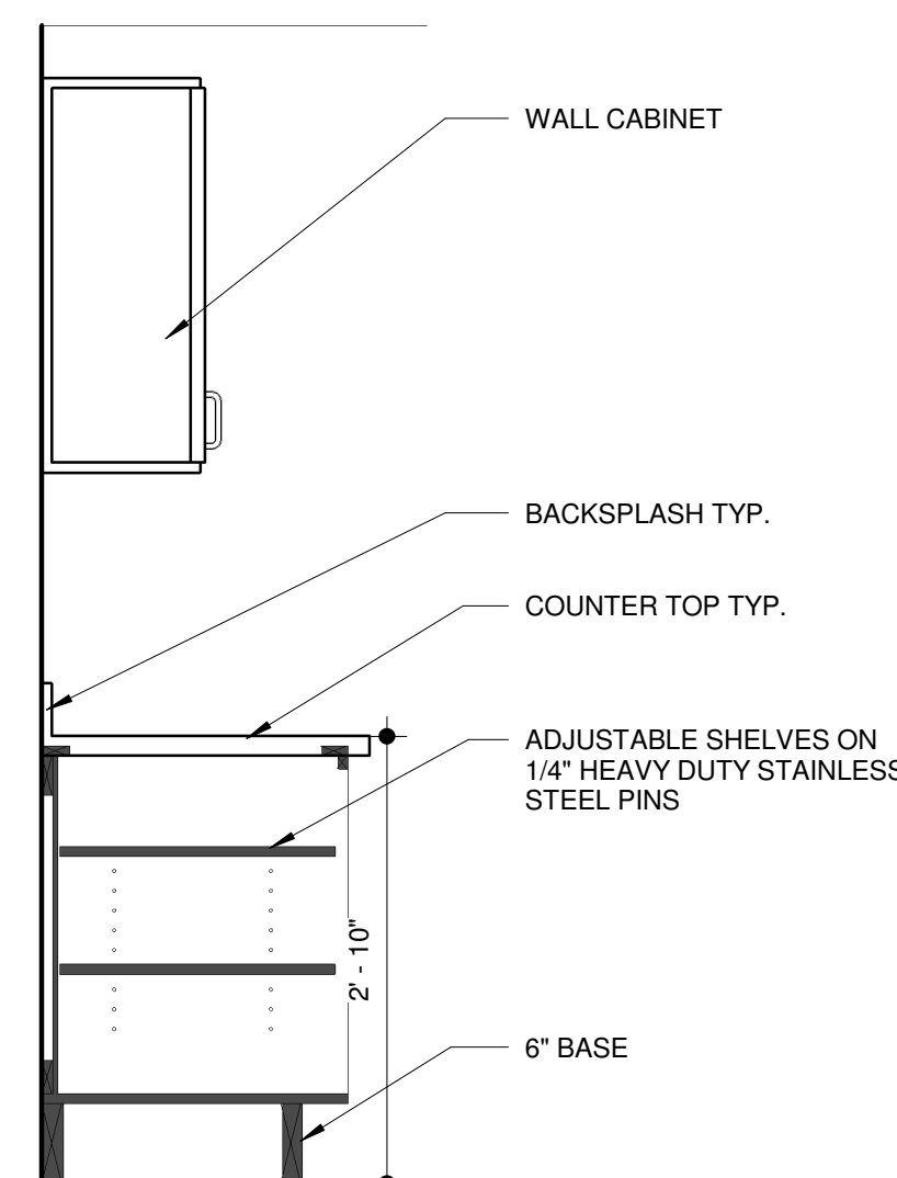
A4 MILWORK SECTION - OPEN BASE CABINET 3/4" = 1'-0"
