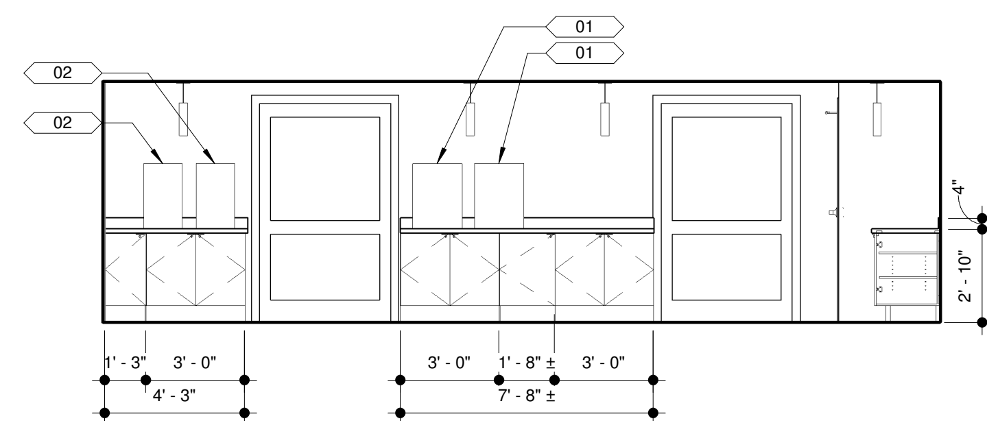
E4 INT ELEV - BREAKFAST PANTRY 1/4" = 1'-0"
