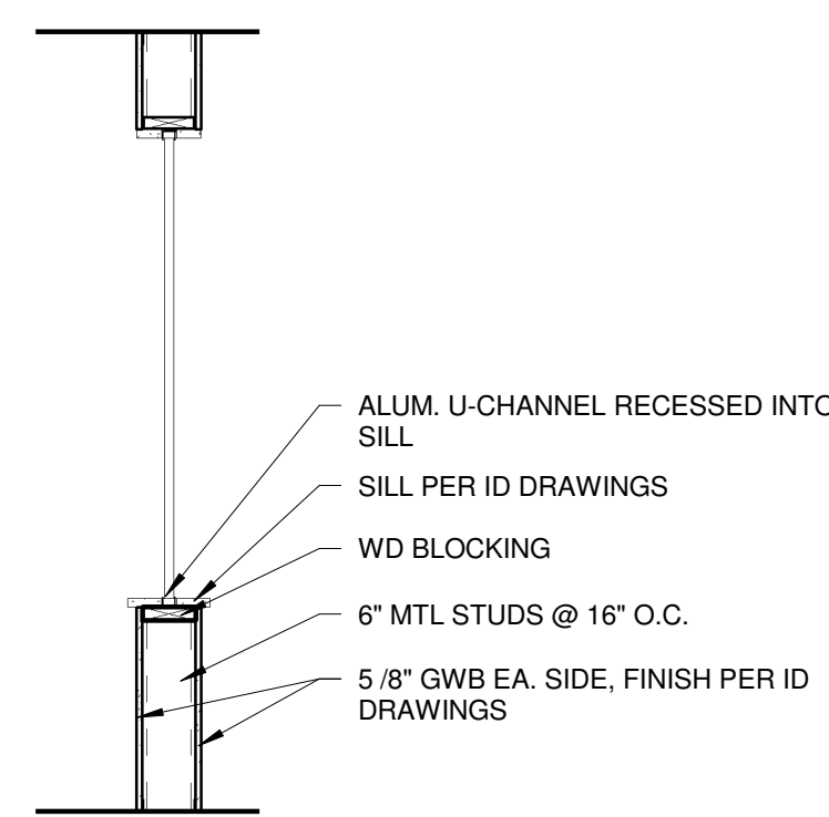
A2 SECTION - GLASS PARTITION 1/2" = 1'-0"
