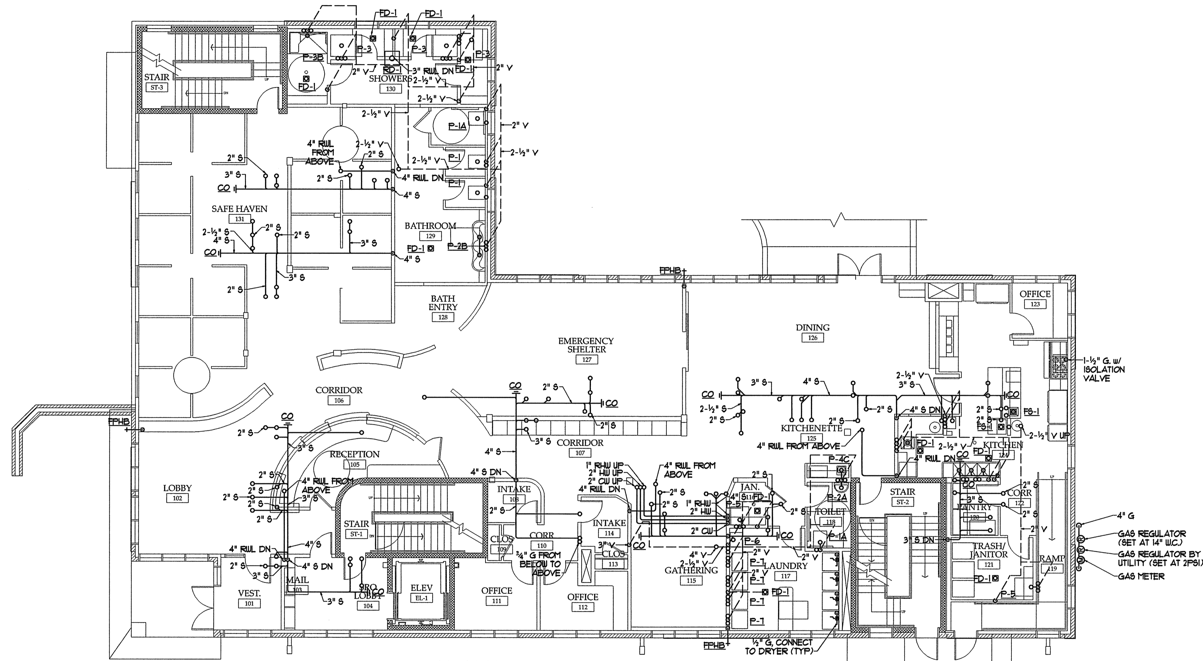
FIRST FLOOR PLUMBING PLAN SCALE - 1/8" = 1'-0"
