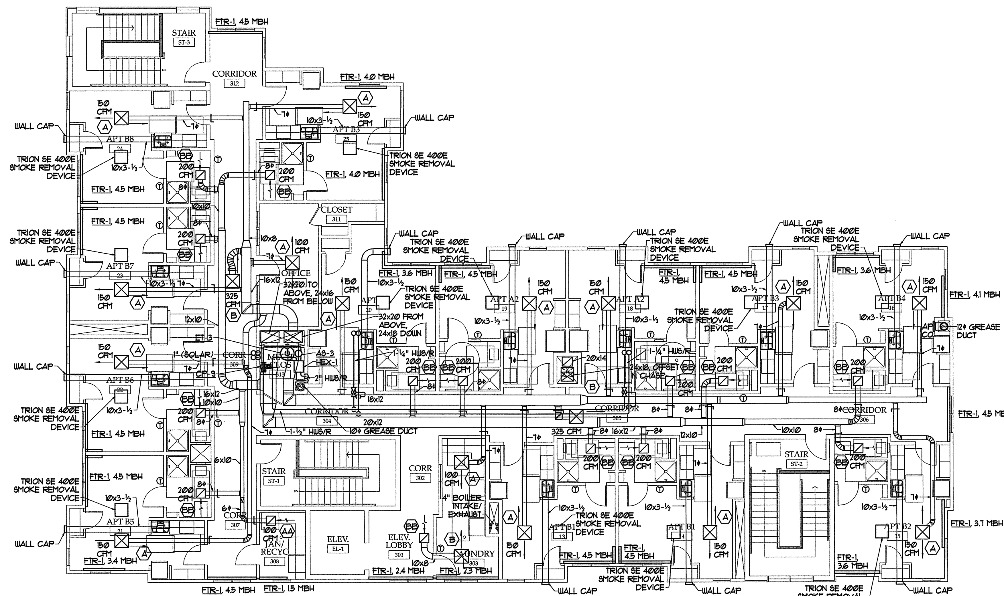
THIRD FLOOR MECHANICAL PLAN SCALE - 1/8" = 1'-0"
