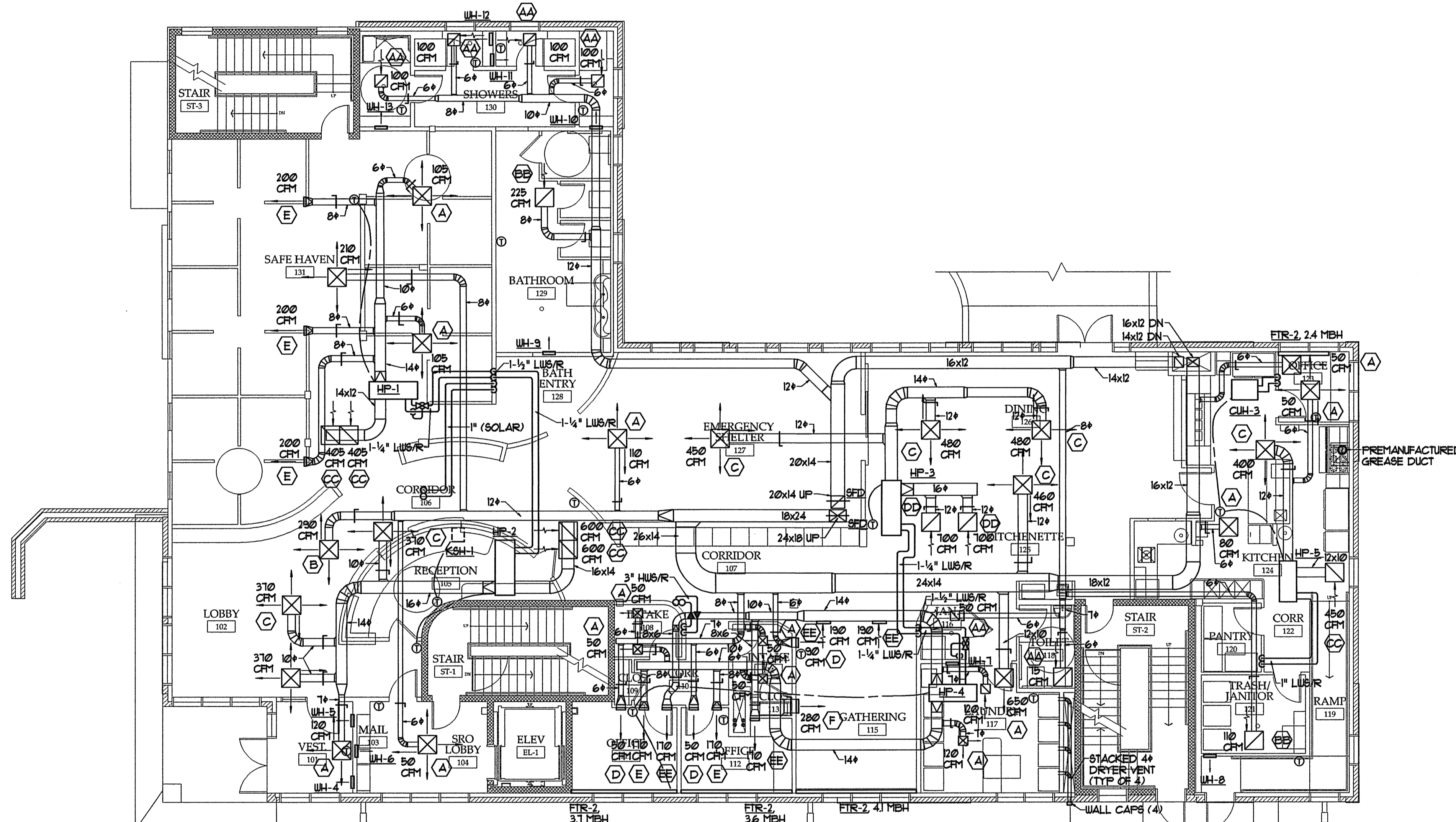
FIRST FLOOR MECHANICAL PLAN SCALE - 1/8" = 1'-0"
