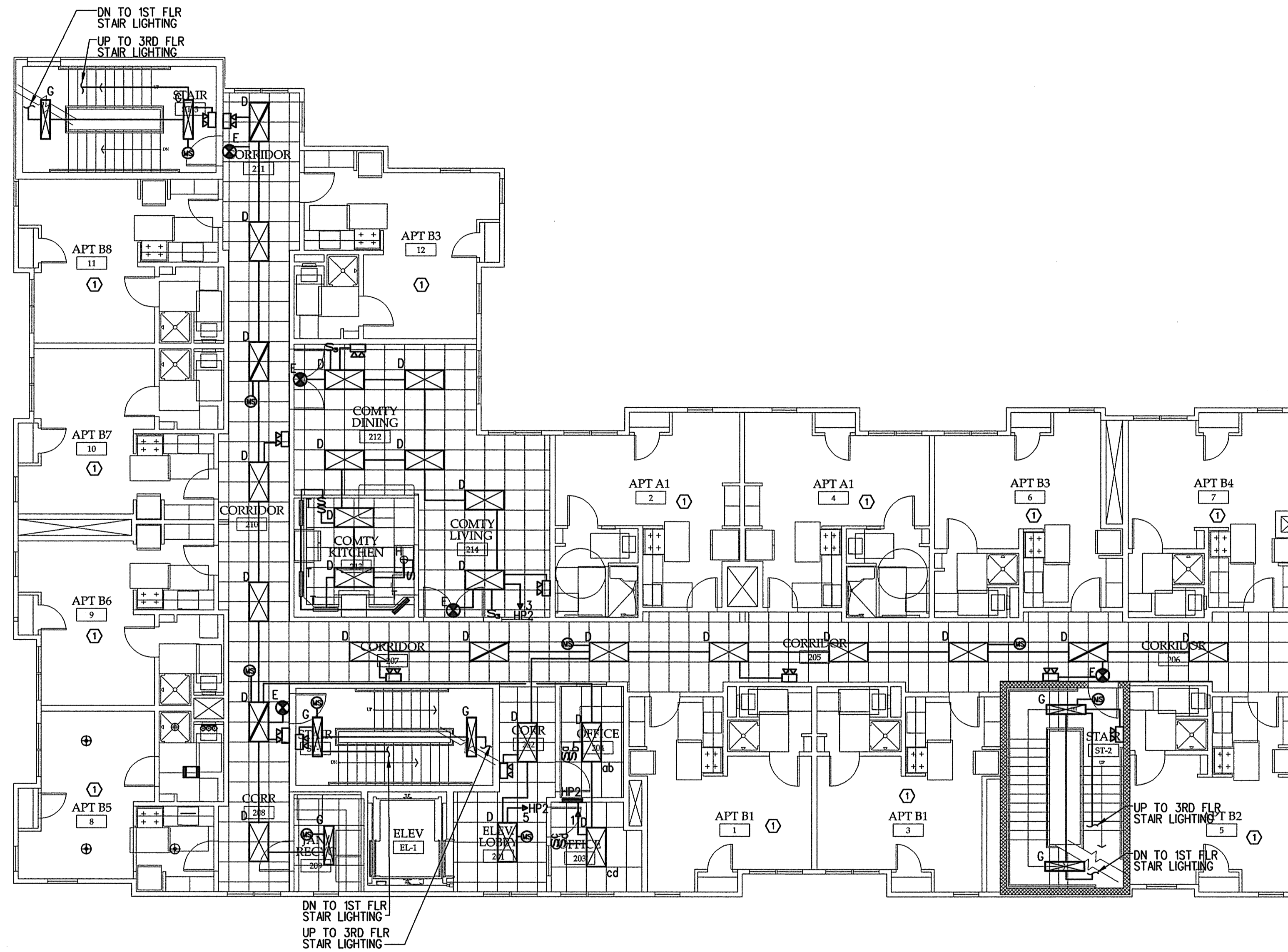
SECOND FLOOR LIGHTING PLAN SCALE: 1/8"=1'-0"
