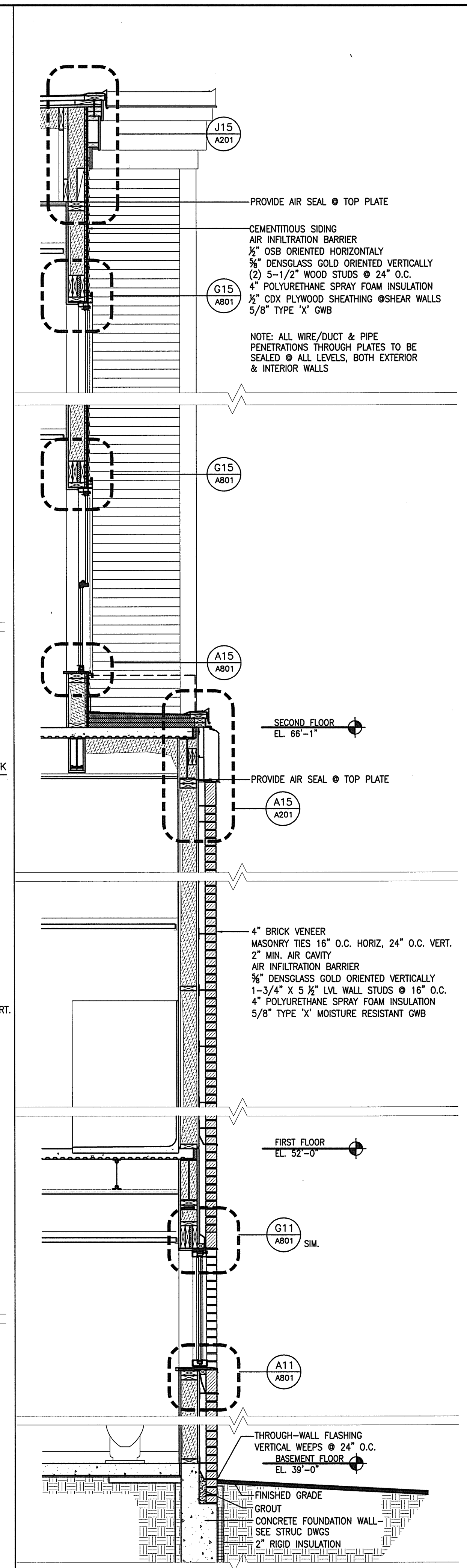
A5 WALL SECTION 1/2"=1'-0" AT LOW ROOF & CANOPY
