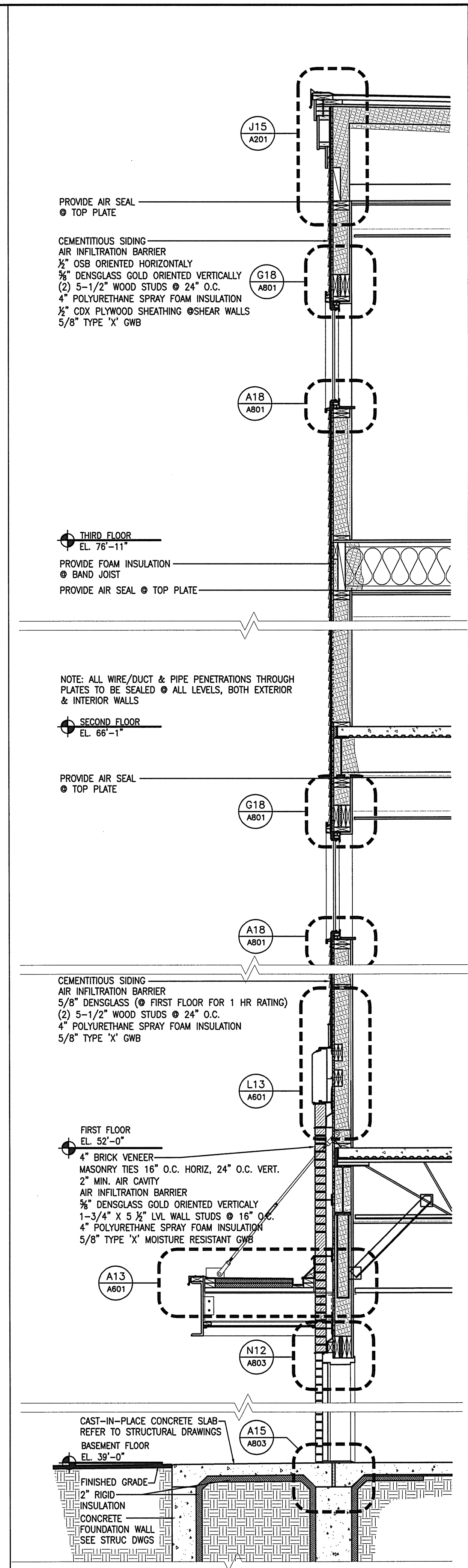
A9 WALL SECTION 1/2"=1'-0"
