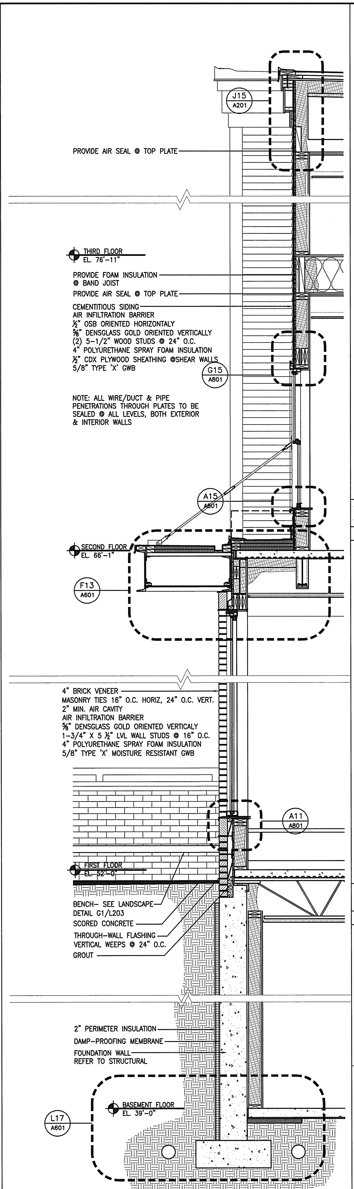
A13 WALL SECTION 1/2"=1'-0" AT LOW ROOF & CANOPY
