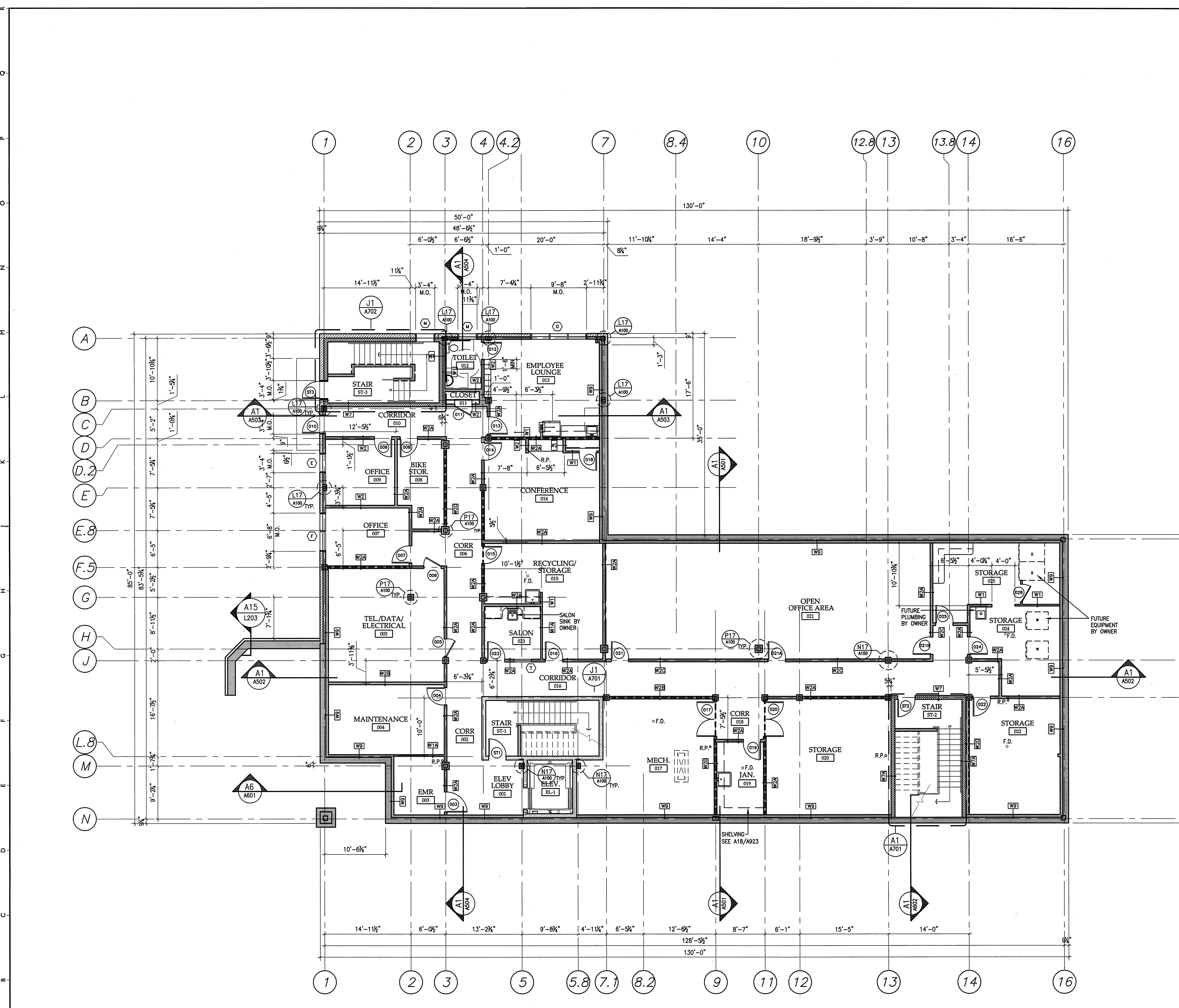
A1 BASEMENT FLOOR PLAN 1/8"=1'-0" 6,131 SF
