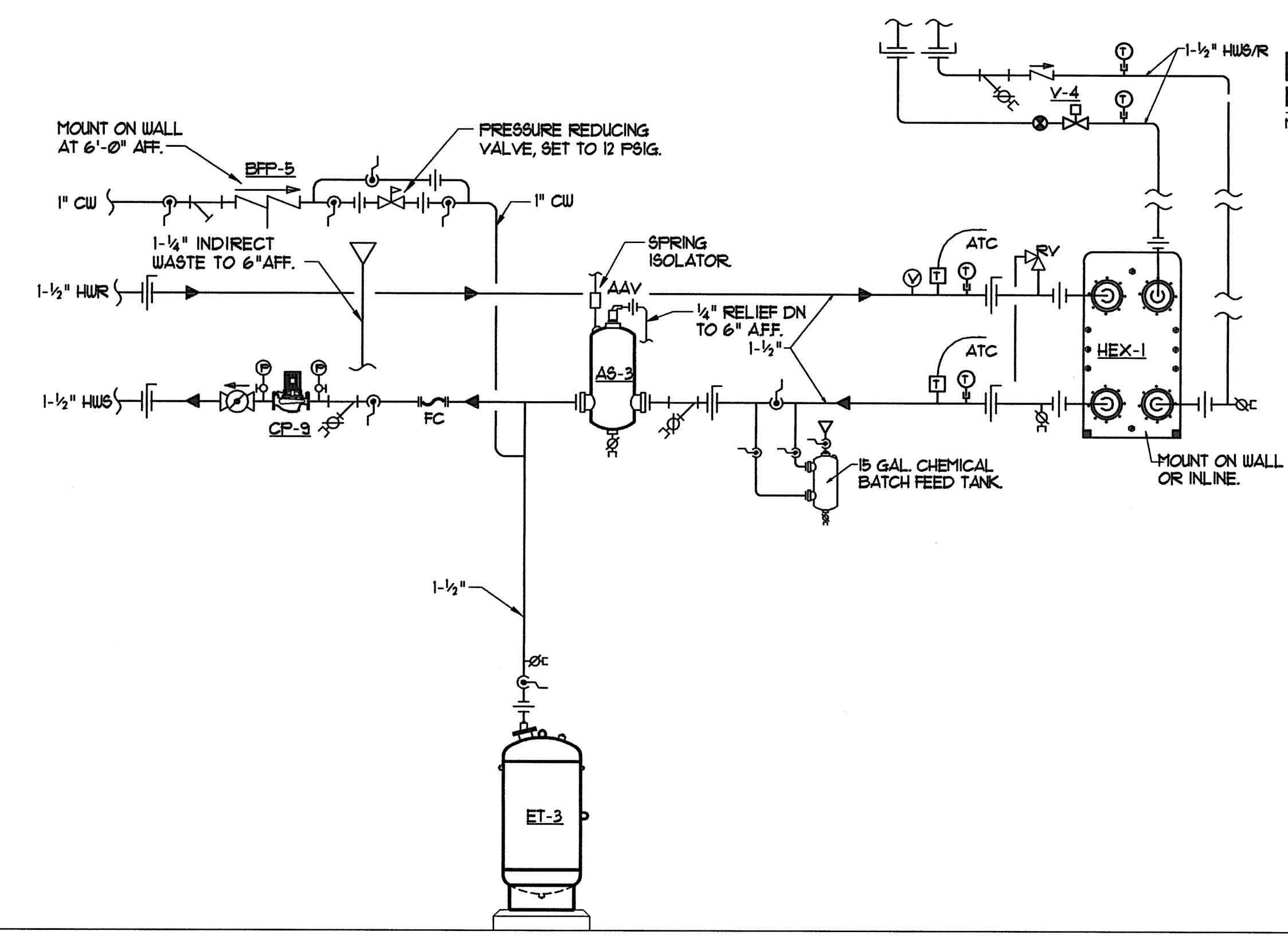
HEAT EXCHAGER PIPING SCHEMATIC NTS
