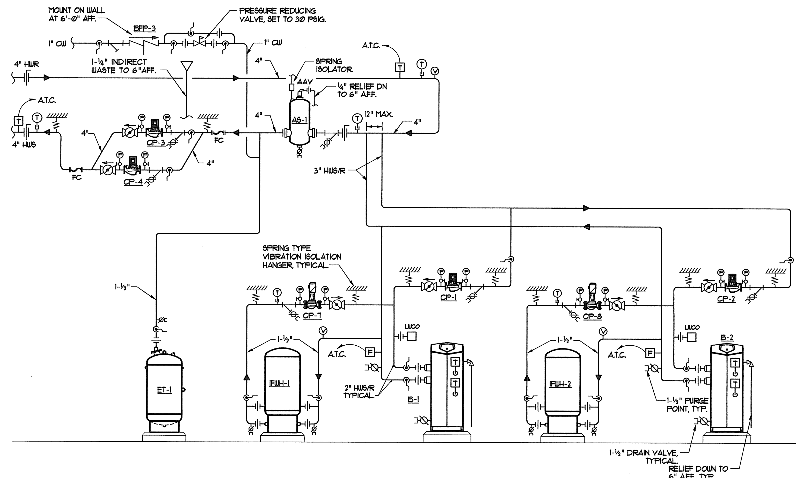
BOILER PIPING SCHEMATIC NTS
