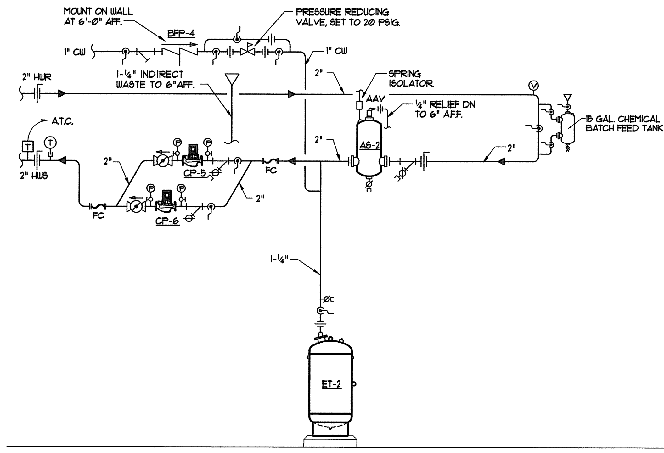
GROUND SOURCE HEAT PUMP PUMPING SCHEMATIC NTS
