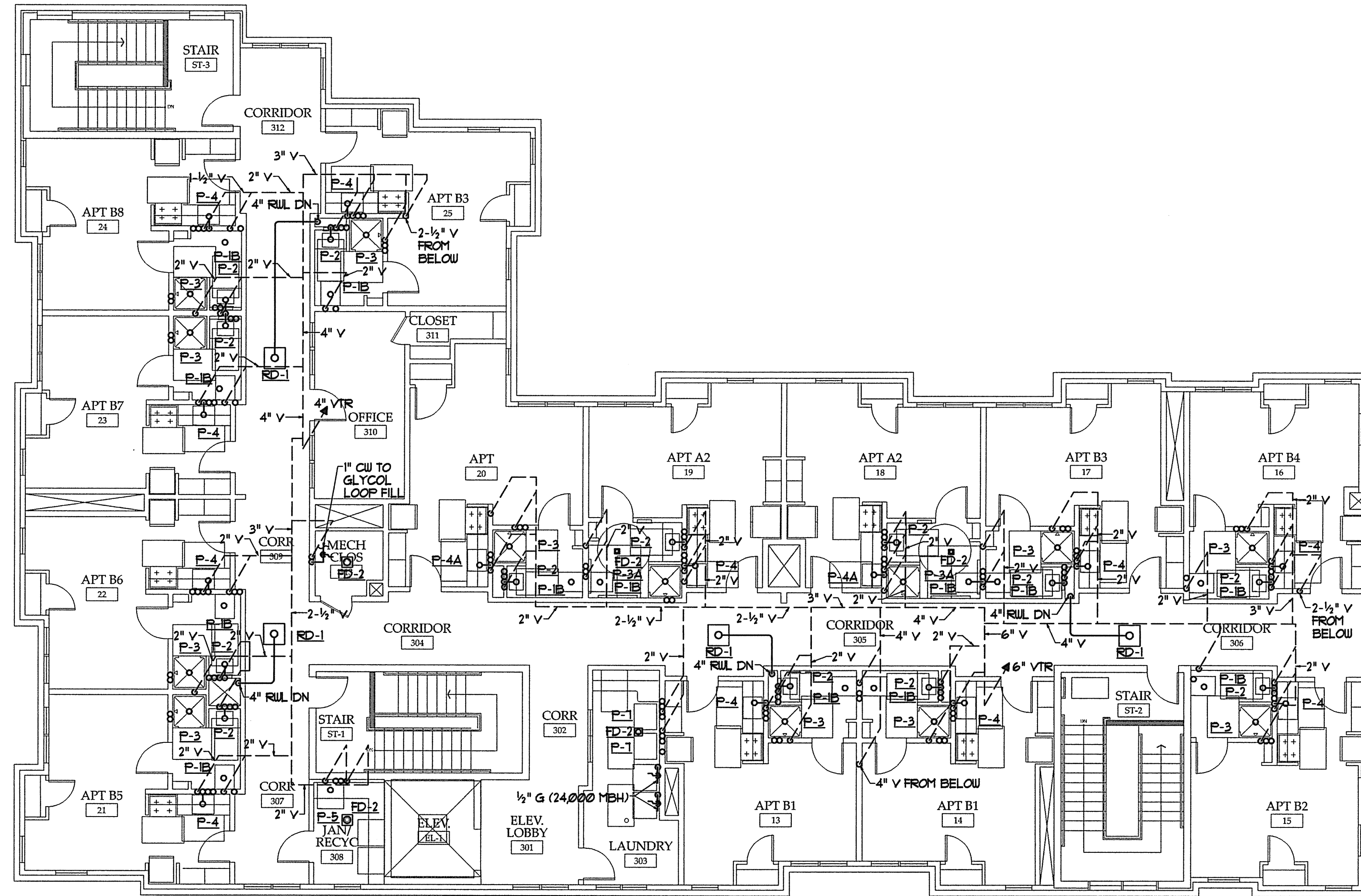
THIRD FLOOR PLUMBING PLAN SCALE - 1/8" = 1'-0"
