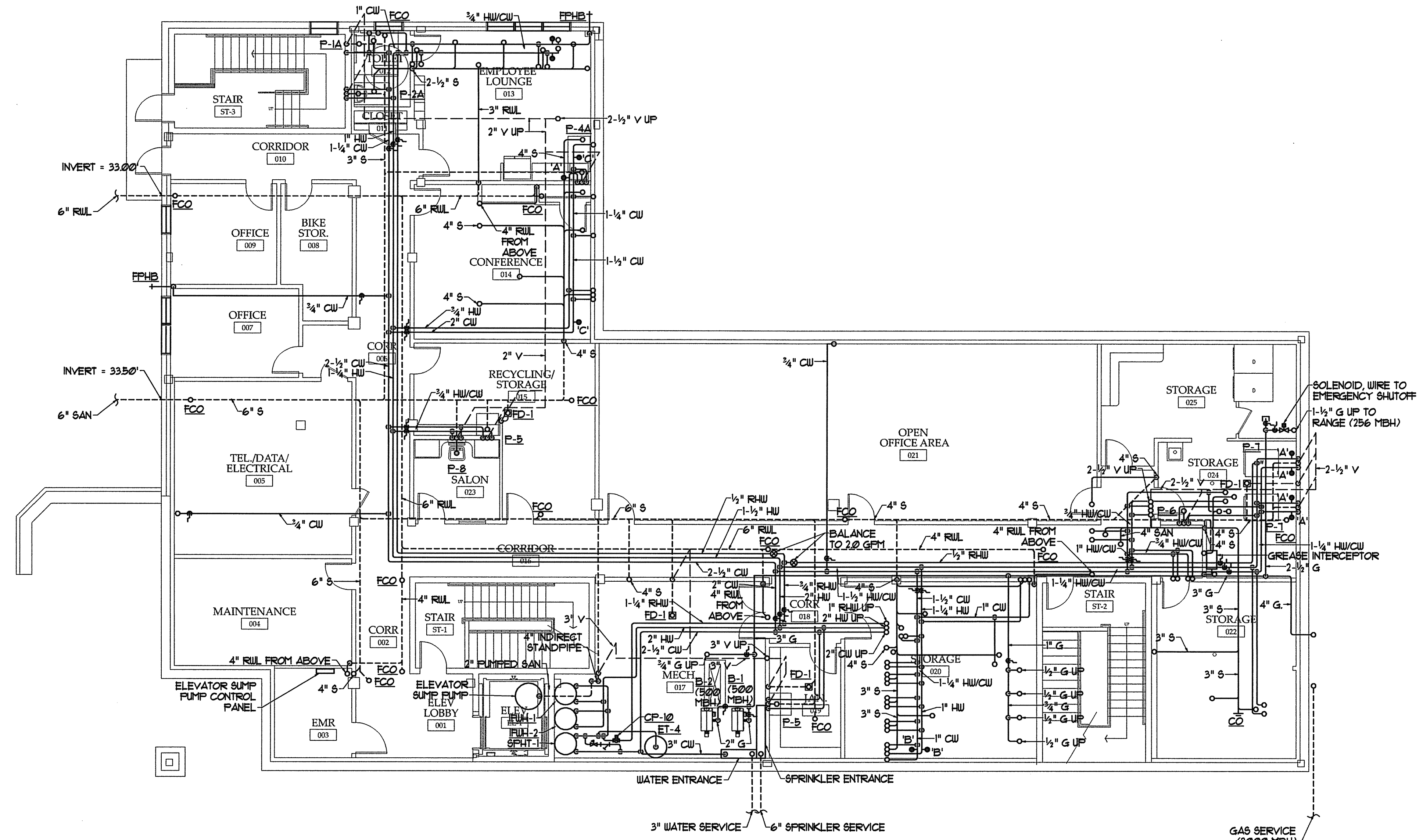
LOWER LEVEL PLUMBING PLAN SCALE - 1/8" = 1'-0"
