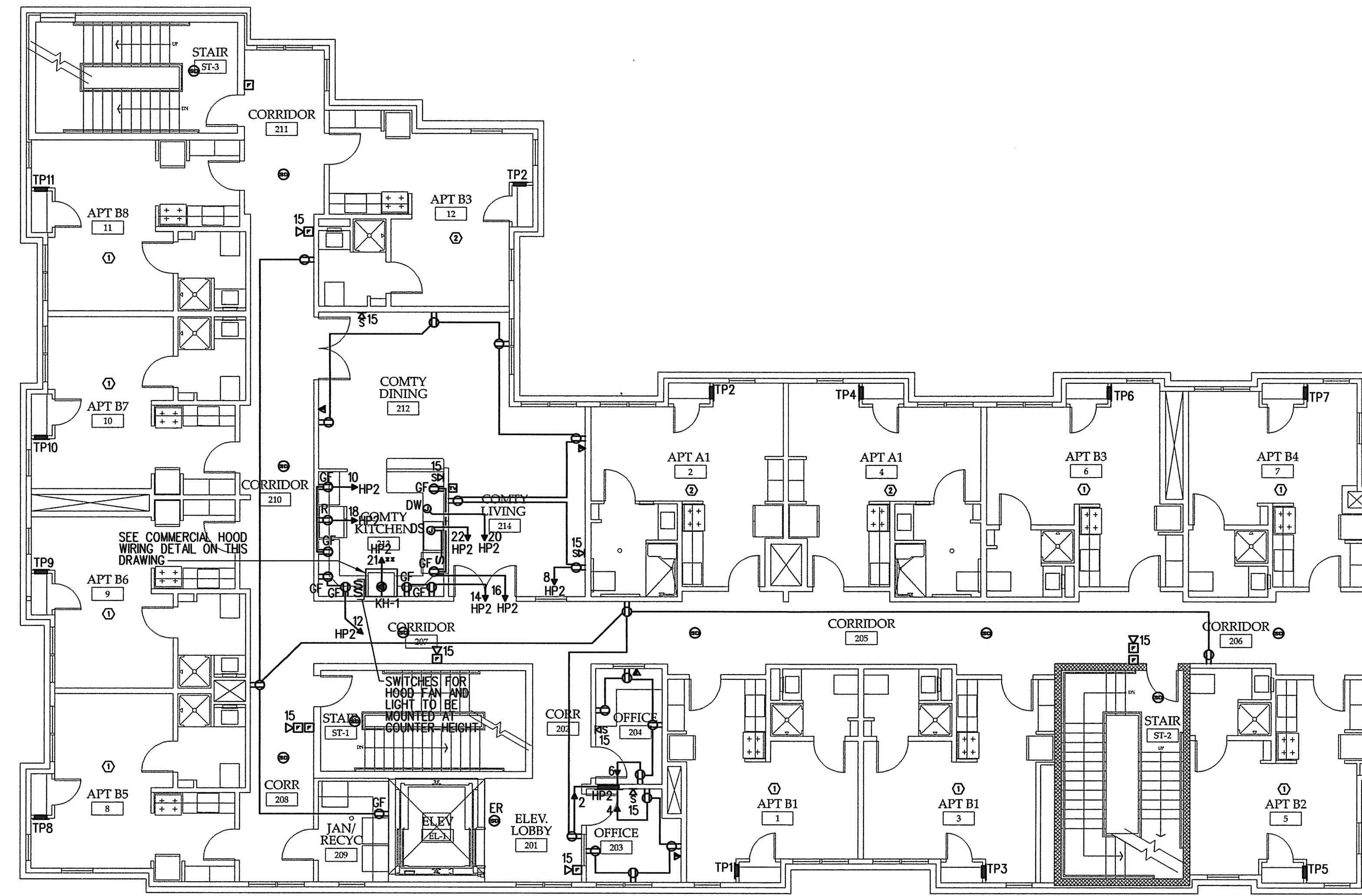
SECOND FLOOR POWER PLAN SCALE: 1/8"=1'-0"
