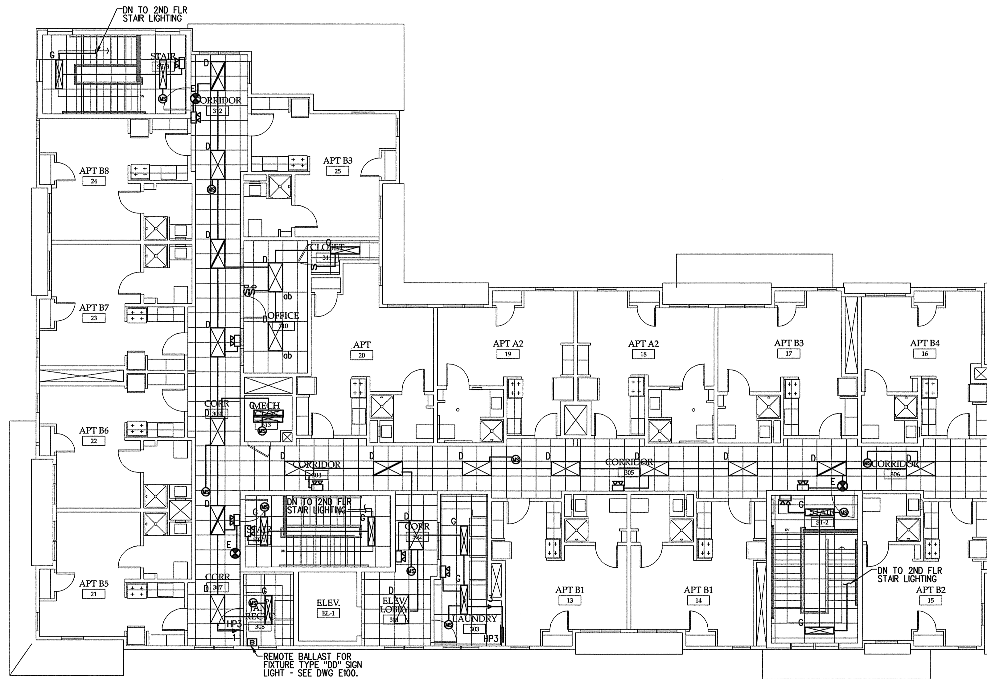
THIRD FLOOR LIGHTING PLAN SCALE: 1/8"=1'-0"
