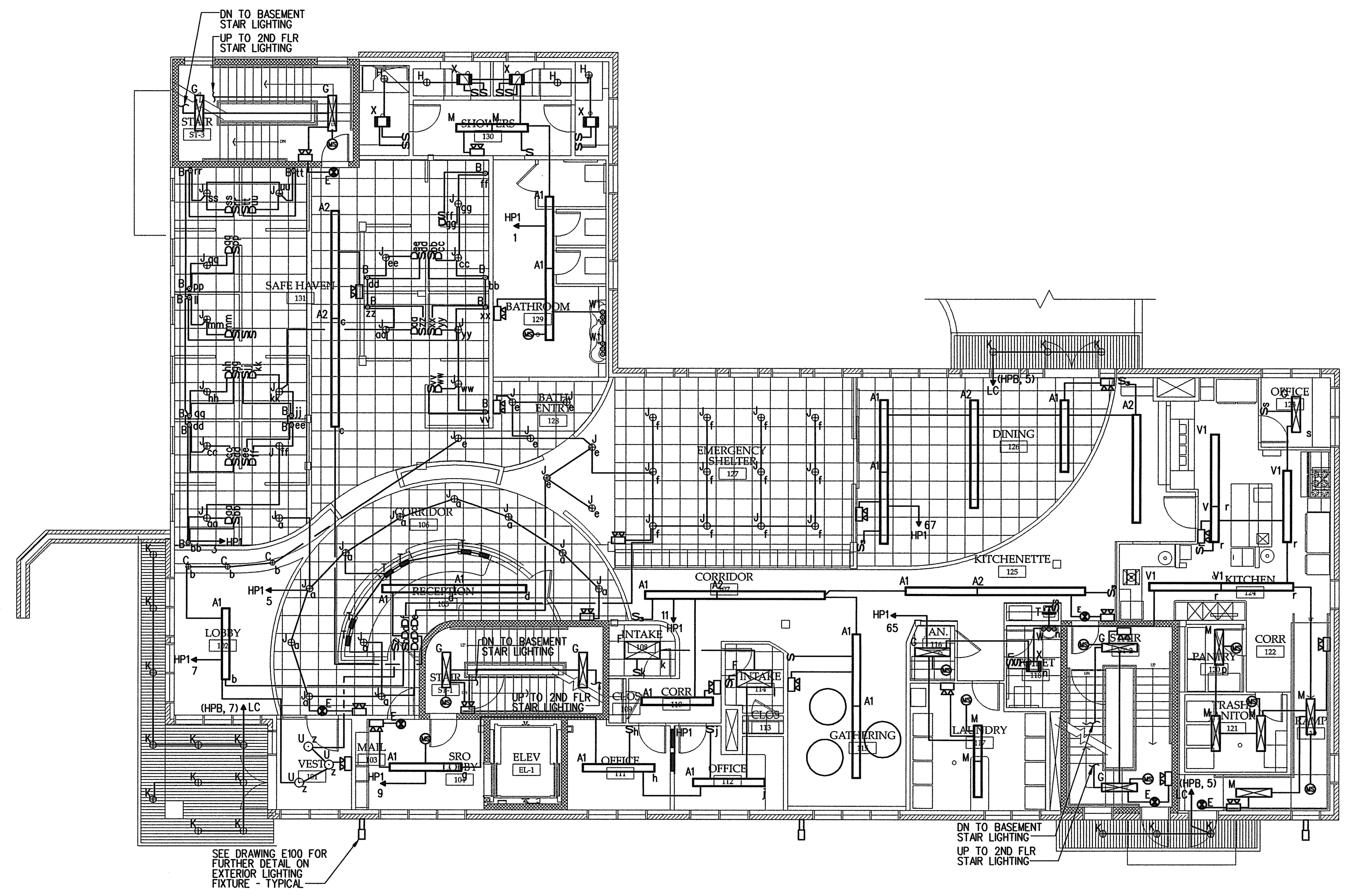
FIRST FLOOR LIGHTING PLAN SCALE: 1/8"=1'-0"
